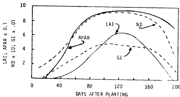
Figure 1. Trajectories of absorbed PAR (APAR), leaf area index (LAI), normalized difference (ND), and greenness index (GI) for well-watered Produr wheat throughout its growing season.
