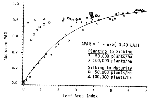
Figure 4. Relation between absorbed PAR and leaf area index for growth (planting to silking) and senescent (silking to maturity) periods of corn.
