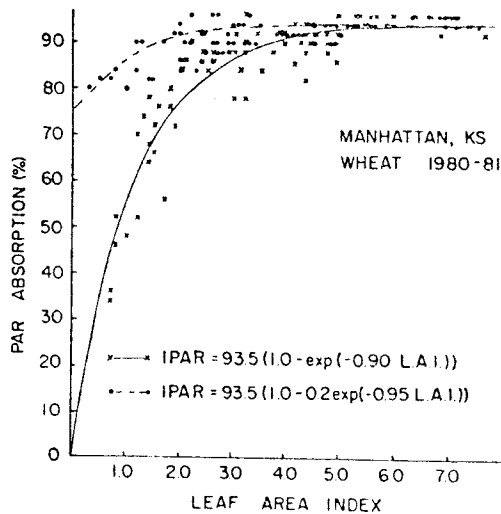
Figure 5. Relation between absorbed PAR and leaf area index for growth (planting to heading) and senescent (heading to maturity) periods of wheat.
