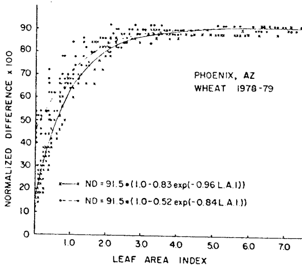
Figure 3. Relation between normalized differences (ND) and leaf area index for the growth (i.e., planting to heading) and senescent (i.e., heading to maturity) periods of wheat.
