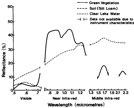
Figure 5.4 Spectral reflectance characteristics of major earth surface cover types (after Bartolucci et al. , 1977)
