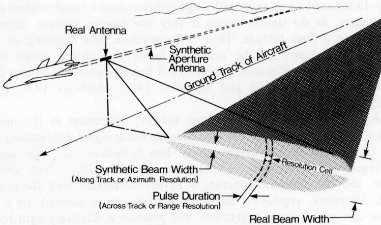
Figure 5.6 Schematic of the basic data collection characteristics of Side-Looking Airborne Radar systems (after Goodyear Aerospace Corp. Staff, 1971)
