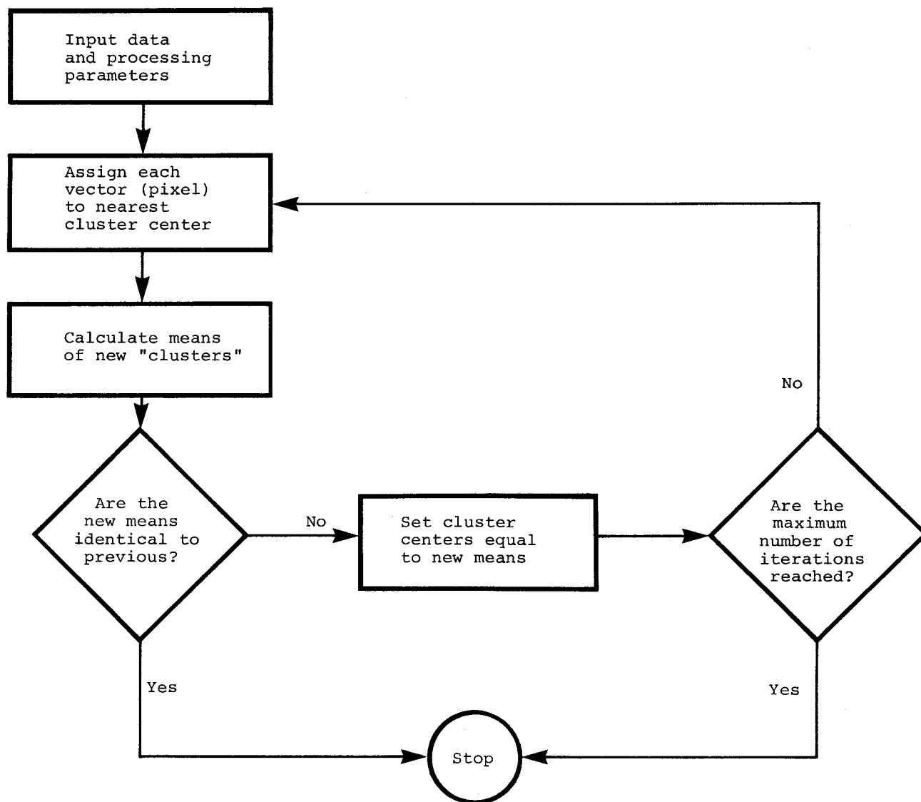
Figure 1. Basic flowchart of clustering algorithm.
