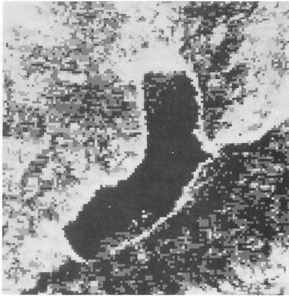
(a) Feature 1: Landsat data in .5-.6 \mu\text{m} band
