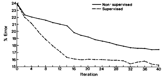
Figure 5a. Comparison of the performance of the supervised and nonsupervised relaxation algorithms. The classification results at a different time were used as ancillary information.
