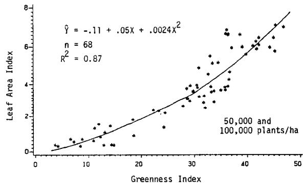
Figure 2. Leaf area index of corn in 1982 as a function of greenness index.
