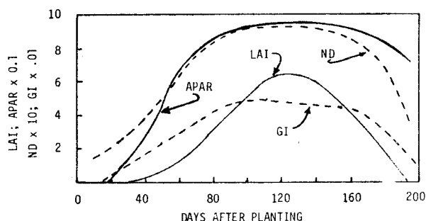
Figure 1. Trajectories of absorbed PAR (APAR), leaf area index (LAI), normalized difference (ND), and greenness index (GI) for well-watered Produr wheat throughout its growing season.
