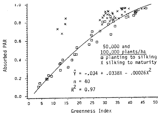
Figure 6. Relation between absorbed PAR and greenness index for growth (planting to silking) and senescent (silking to maturity) periods of corn.
