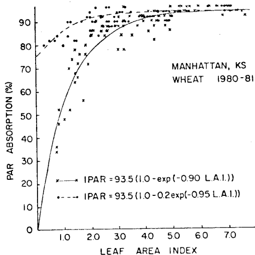
Figure 5. Relation between absorbed PAR and leaf area index for growth (planting to heading) and senescent (heading to maturity) periods of wheat.
