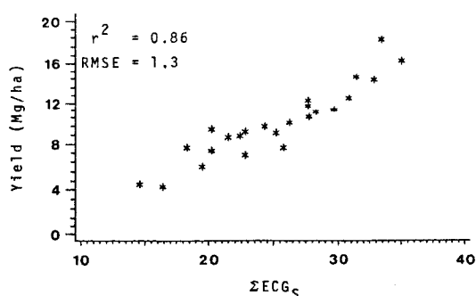
Figure 8. Grain yields of corn in 1982 as a function of the energy-crop growth (ECG) model. The ECG model combines the concept of absorbed PAR with moisture stress and temperature functions to describe crop growth and yield.
