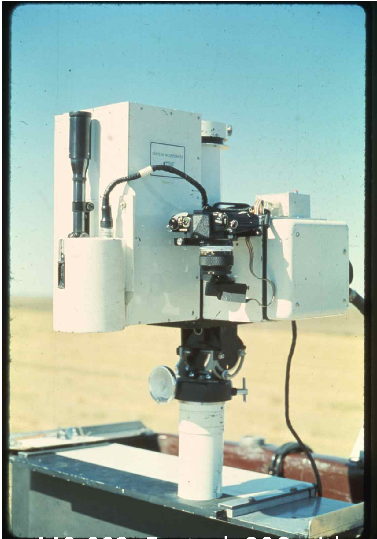
440-002: Exotech 20C with PRT-5 & Camera on pedestal
