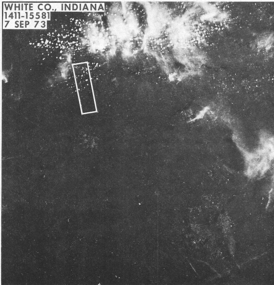
Figure 10.- ERTS-1 frame 1411-15581 (1:250,000).
