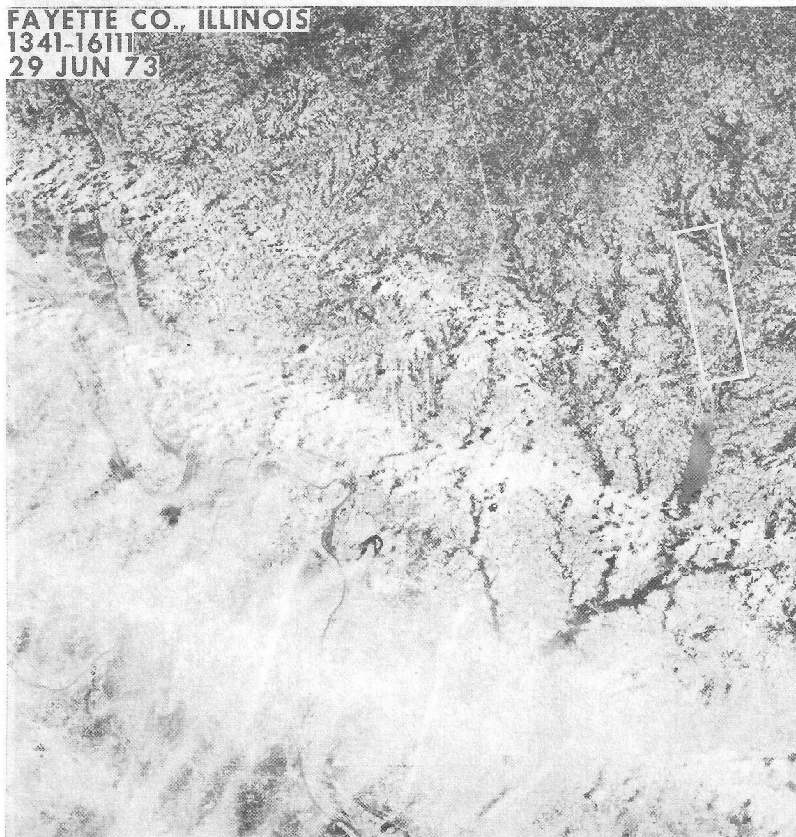
Figure 17.- ERTS-1 frame 1341-16111 (1:250,000).
