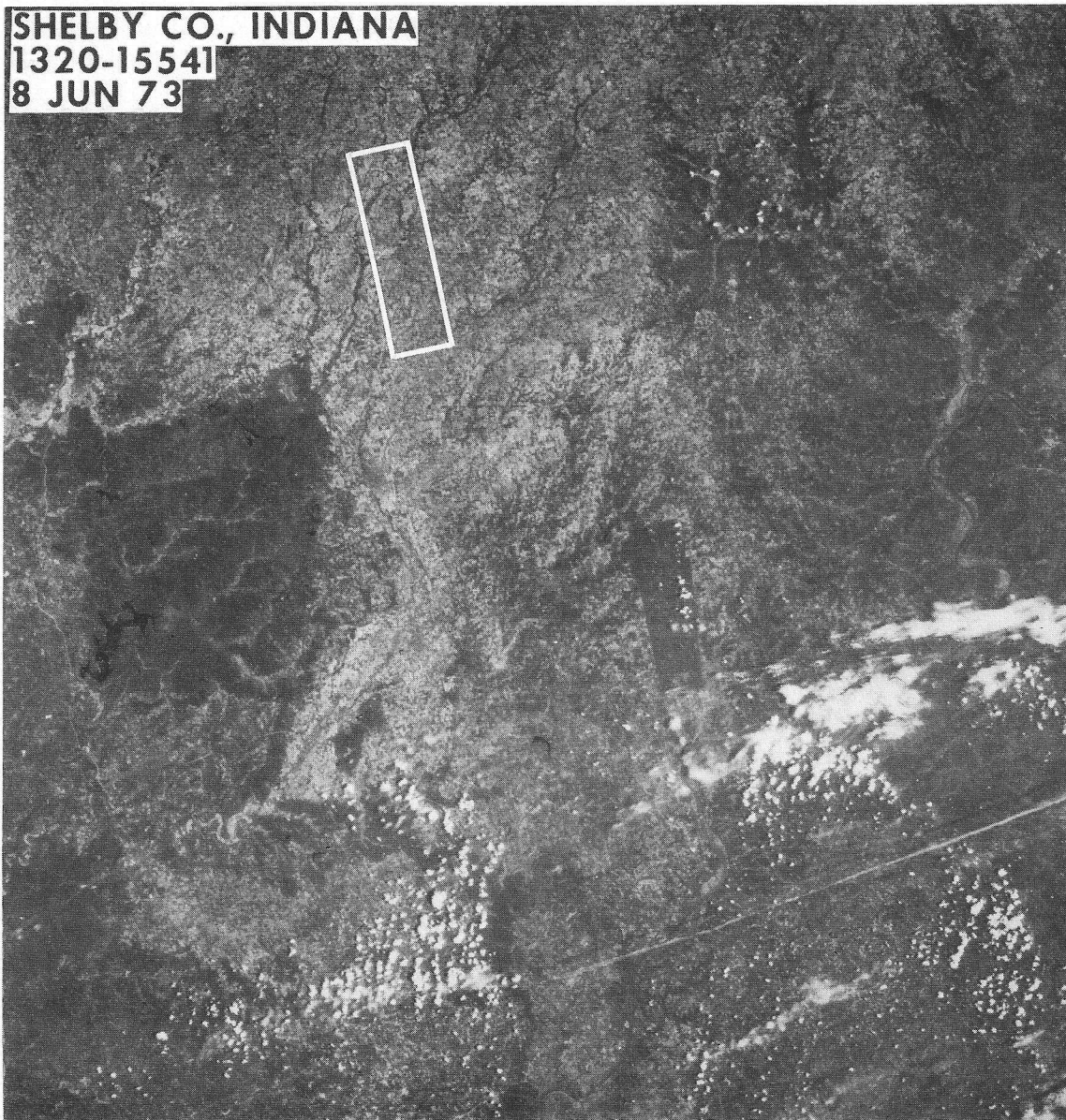
Figure 5.- ERTS-1 frame 1320-15541 (1:250,000).
