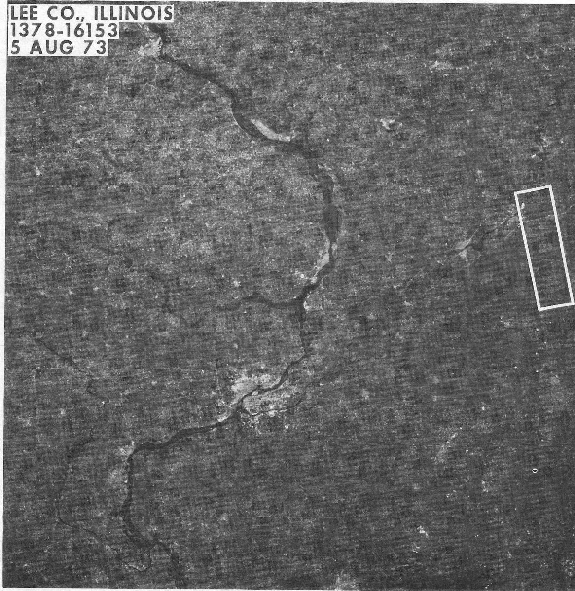
Figure 23.- ERTS-1 frame 1378-16153 (1:250,000).
