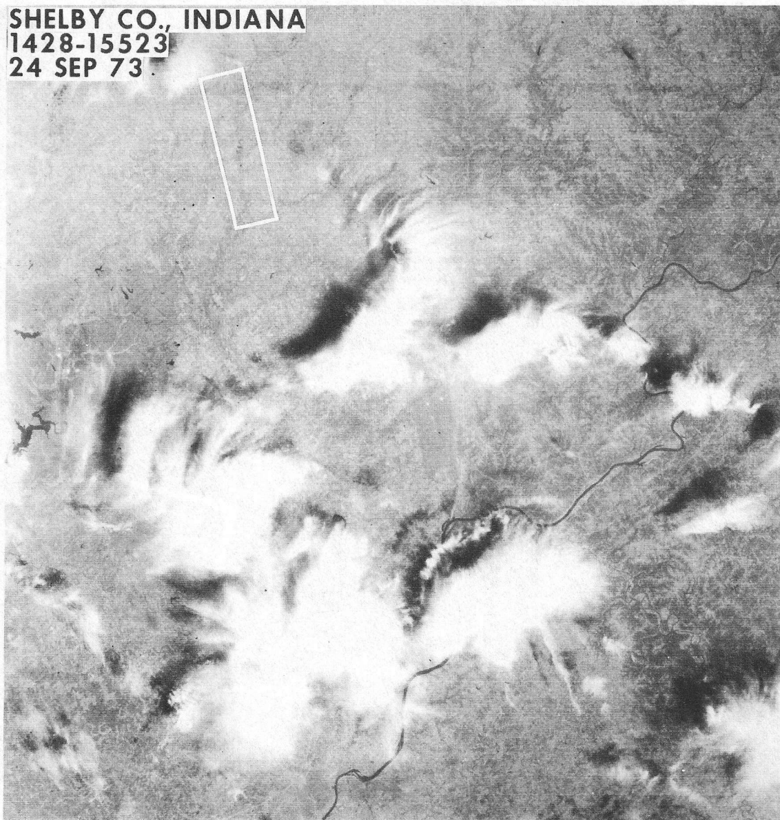
Figure 7.- ERTS-1 frame 1428-15523 (1:250,000).
