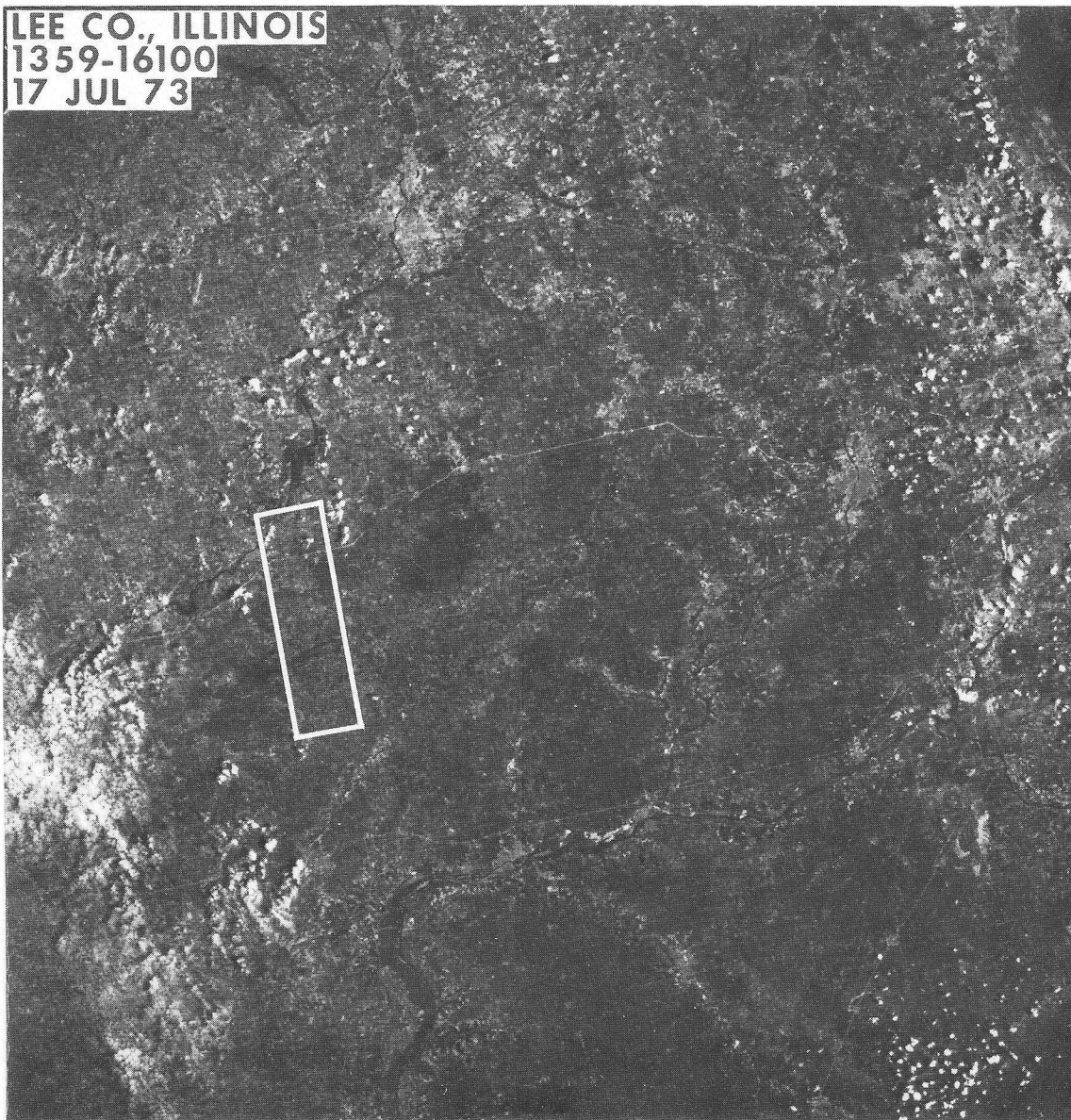
Figure 21.- ERTS-1 frame 1359-16100 (1:250,000).
