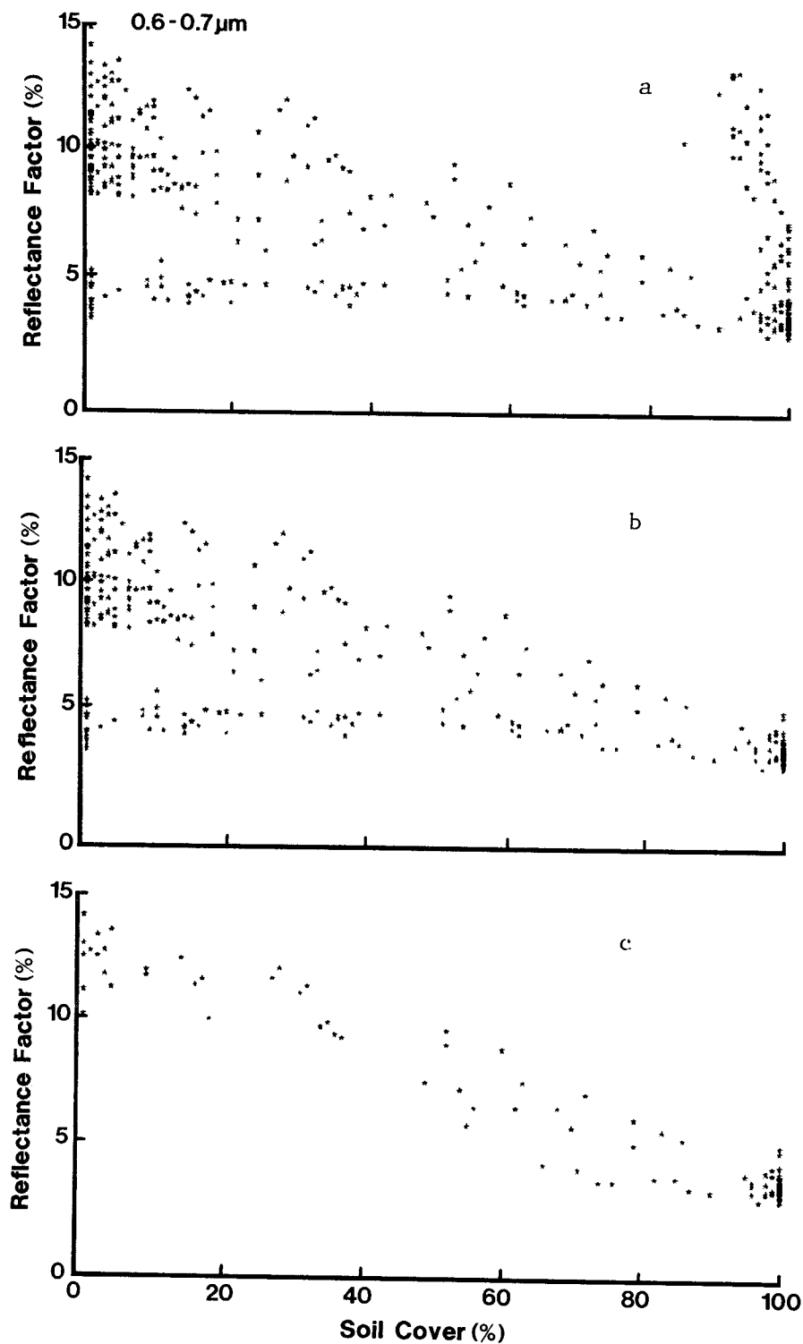
Figure 2. Relationship of RF in the red wavelength region (0.6-0.7 \mu\text{m} ) to percent soil cover in 1979 (a) full data set (b) minus dates including senescing vegetation (c) minus dates including senescing vegetation and/or moist soil. (Chalmers silty clay loam)
