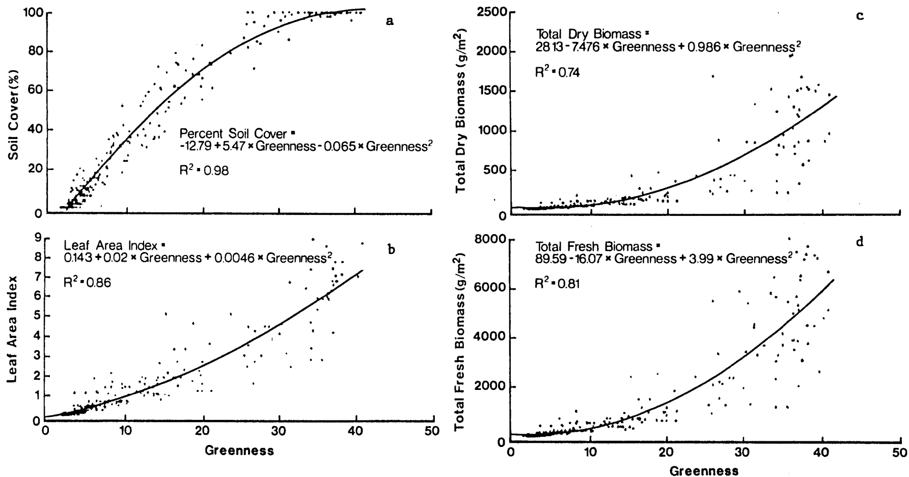
Figure 7. Plots of four agronomic variables versus greenness (a) percent soil cover (b) leaf area index (c) total dry biomass (d) total fresh biomass. (Chalmers silty clay loam)
