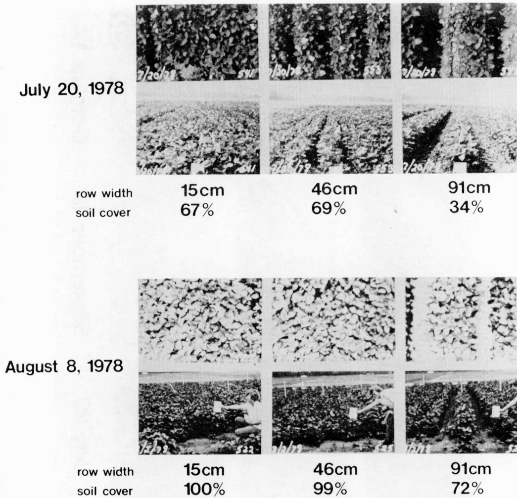
Figure 11. Changes in soil cover over three row widths on two dates.
