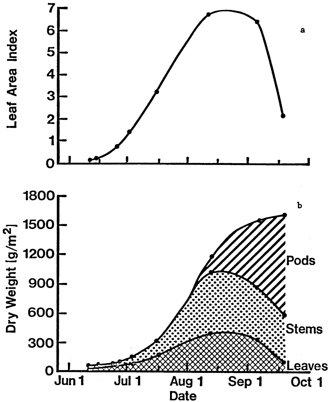
Figure 8. Seasonal changes in (a) leaf area index and (b) soybean canopy components for the May 24 planting date on Chalmers silty clay loam.
