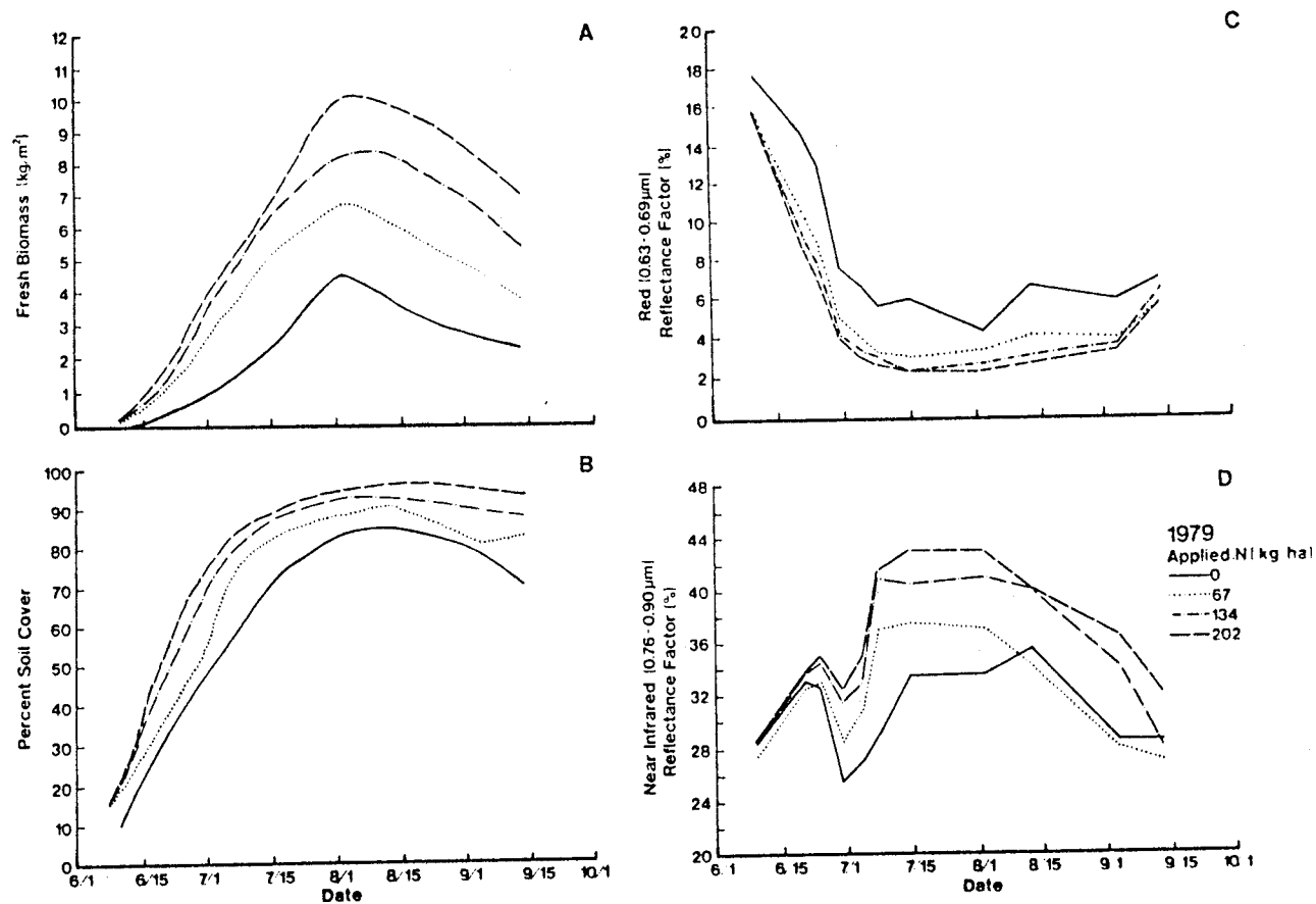
Figure 3. Temporal changes in (A) fresh biomass, (B) percent soil cover, (C) red (0.63-0.69 \mu m) reflectance factor for corn canopies under four N treatment levels in 1979.
