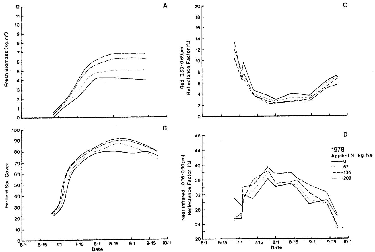
Figure 2. Temporal changes in (A) fresh biomass, (B) percent soil cover, (C) red (0.63-0.69 \mu m) and (D) near infrared (0.76-0.90 \mu m) reflectance factor for corn canopies under four N treatment levels in 1978.
