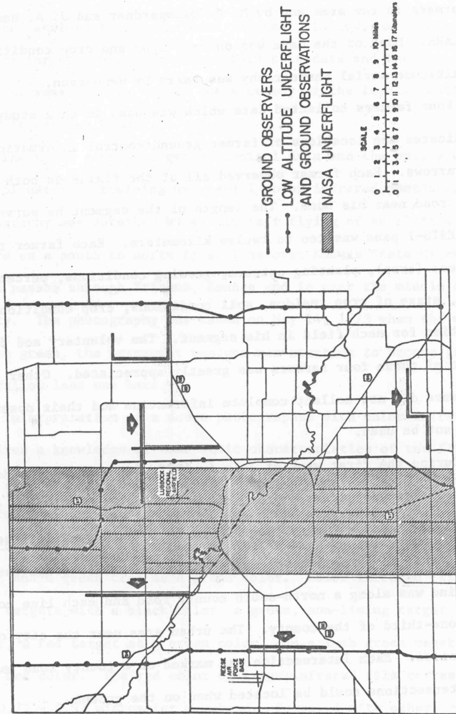
Figure 1. Location of ground information used in the analysis of Lubbock County, Texas.
