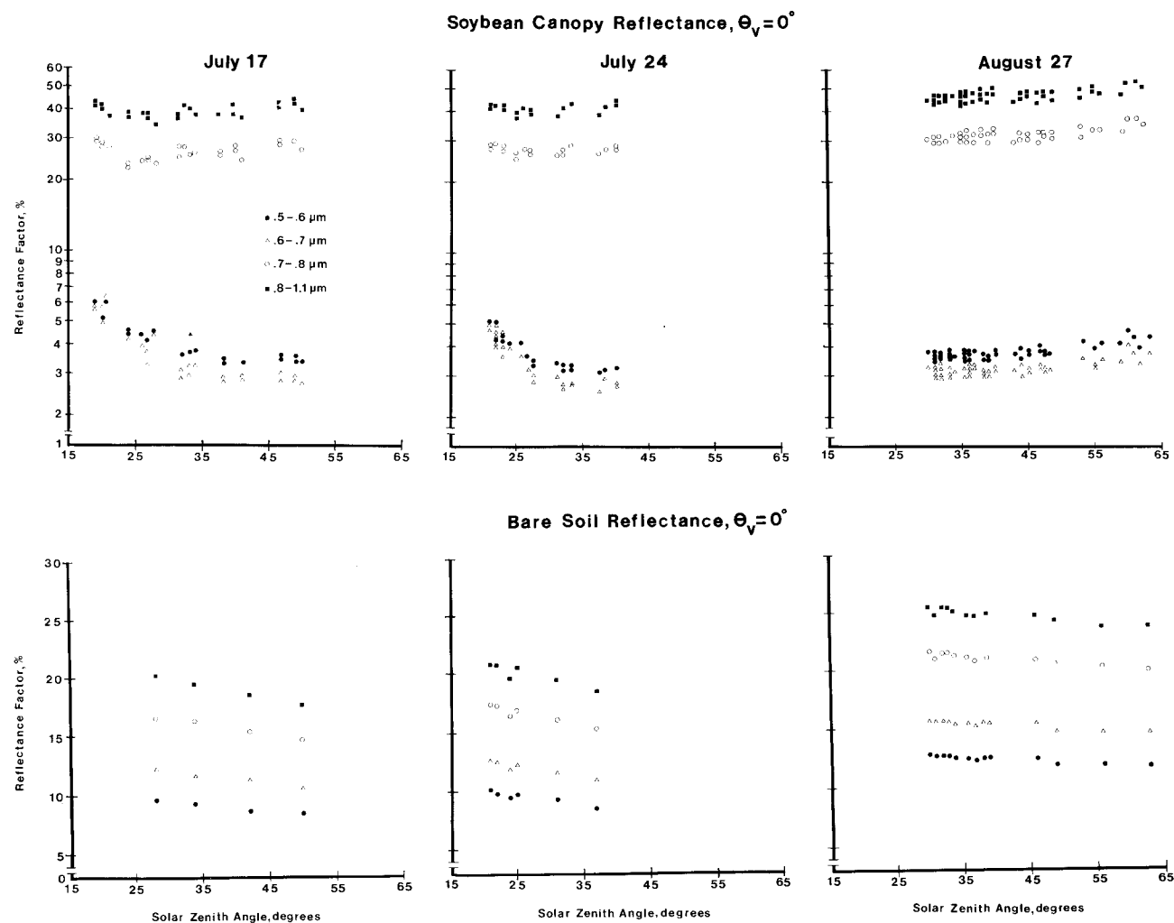
Figure 5. Relationships of soybean canopy and bare soil reflectance factors and solar zenith angle on three days for a nadir looking sensor.
