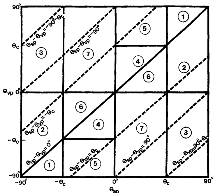
Figure 7. Model diagram of \theta_{sp} , \theta_{vp} plane. Numbered regions within solid lines indicate areas of nearly constant reflectance defined by \theta_{sp} , \theta_{vp} and \theta_c (see Table 3). Dashed lines represent equal values of \theta_{sp} - \theta_{vp} angles.
