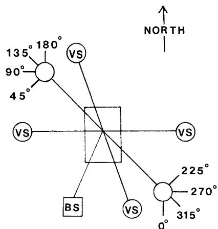
Figure 1. Diagram of boom positions for measurement of reflectance hemispheres. VS = vertically viewed soybeans. BS = vertically viewed bare soil.
