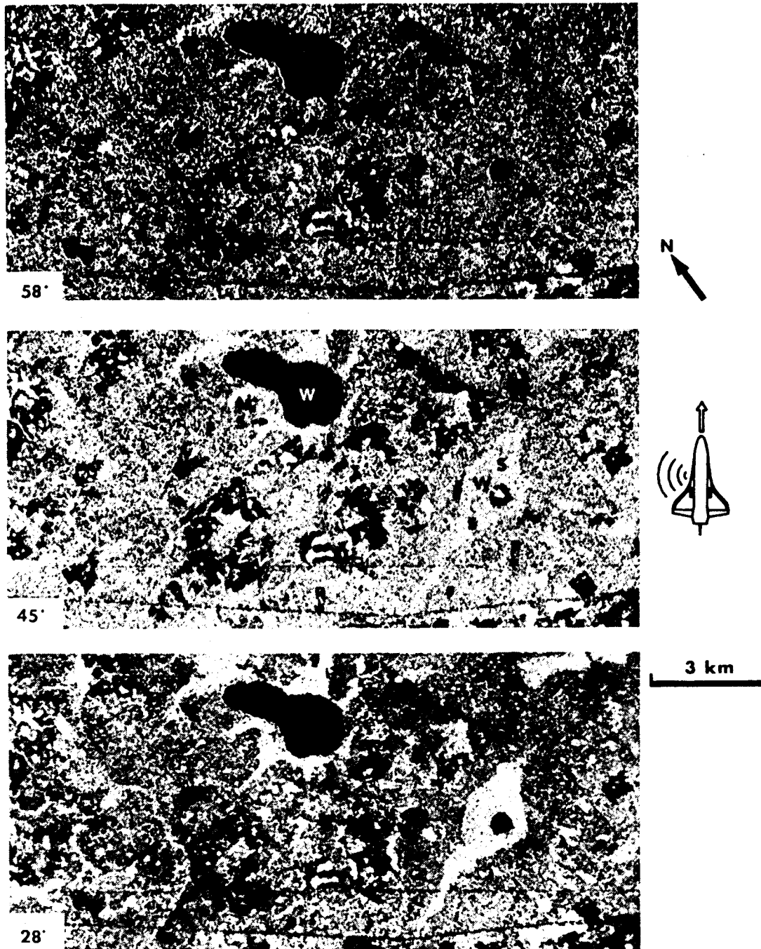
Figure 2. Multiple incidence-angle SIR-B data of the Florida test site. The light-toned areas of deciduous swampland forest are very distinct on the 28° image (bottom), but cannot be differentiated from the surrounding slash pine on the 58° image (top). The center image was obtained at an incidence angle of 45°. W = Water; F = Slash Pine Forest; S = Deciduous Swampland; C = Clearcut; R = Road; and P = Powerline.
