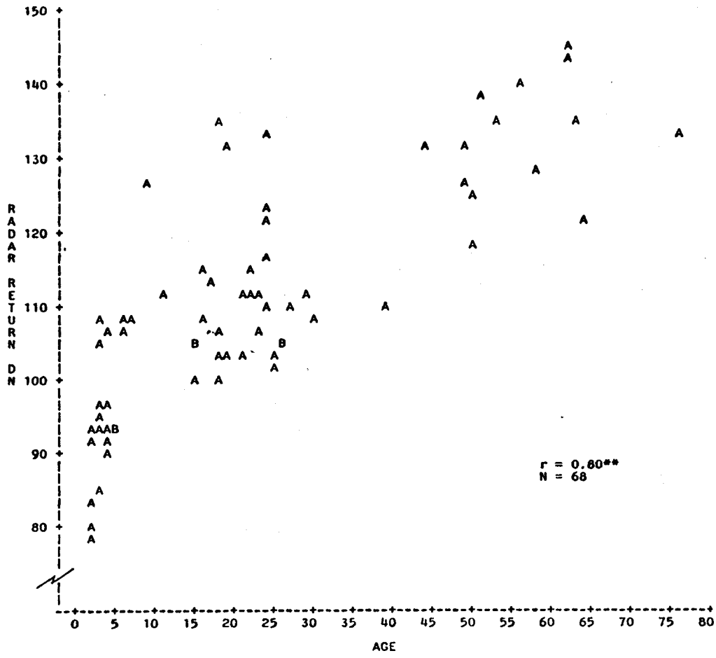
Figure 1. Plot of SIR-B radar backscatter versus age of slash pine. (N = 68 stands; r = 0.80**).
