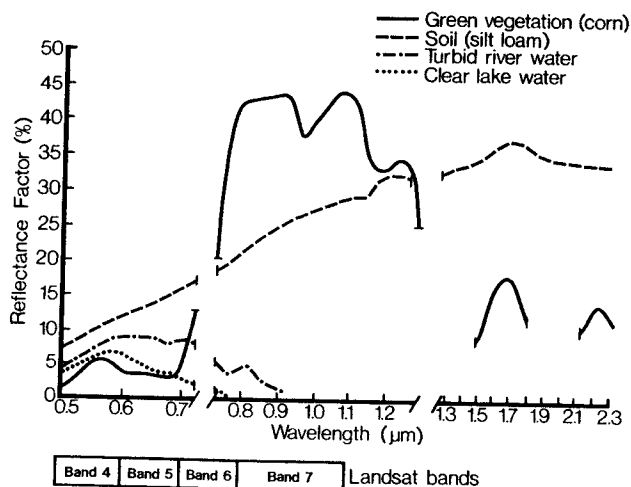
Figure 1. Spectral Reflectance Characteristics of Major Earth-Surface Materials.
