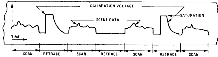
Figure 2. Representation of Output Signal from Landsat MSS System. Response curves show four scan and three retrace movements, the latter including the maximum (saturation) and minimum calibration signals.
