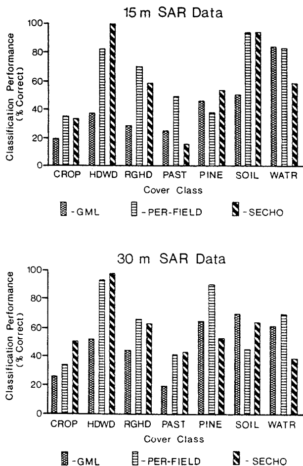
Figure 4. Classification performances by cover class for the three classifiers, and for both the SAR 15 m and 30 m data sets.
