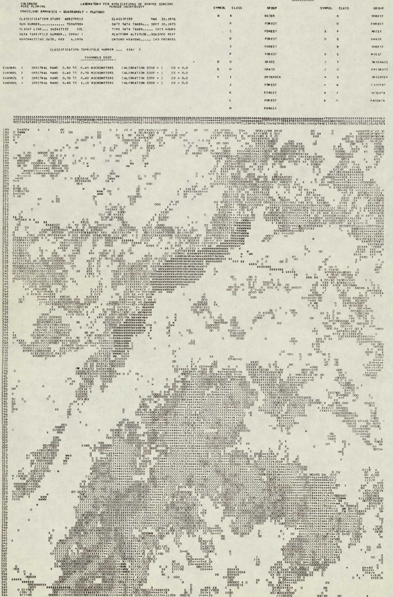
Figure C.8. Classification map for Platoro quadrangle which emphasizes the grassland cover types.
