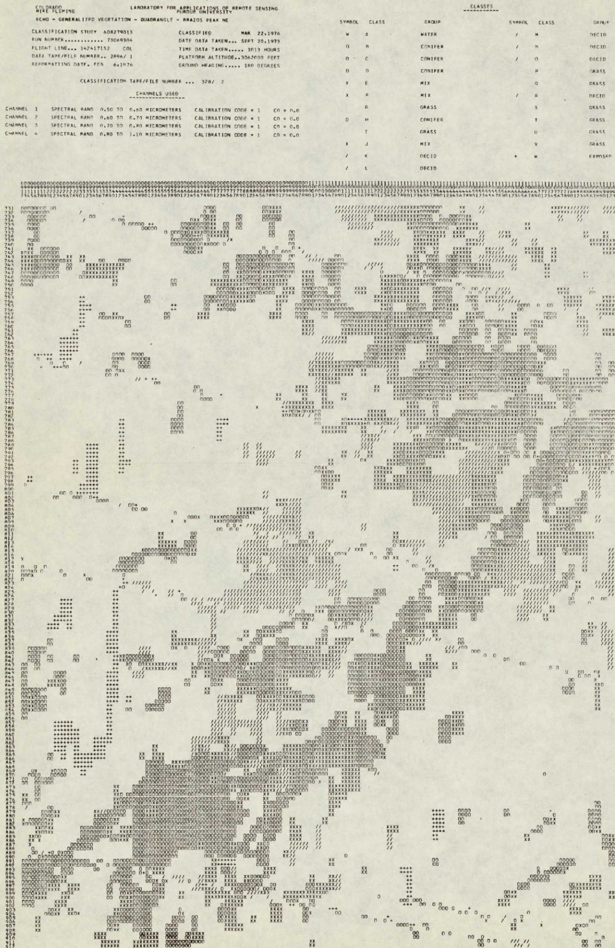
Figure C.17. Classification map for Brazos Peak NE quadrangle showing the generalized vegetation classes when the ECHO classifier was utilized.
