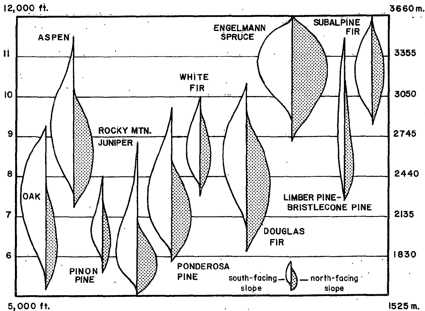
Figure A.2. Distribution of dominant tree species along an elevation gradient. The relative abundance is shown with respect to north- and south-facing slopes.
