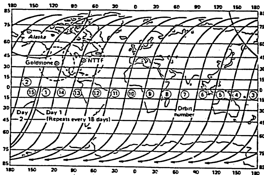
Figure 5. The Landsat space orbit diagram.
