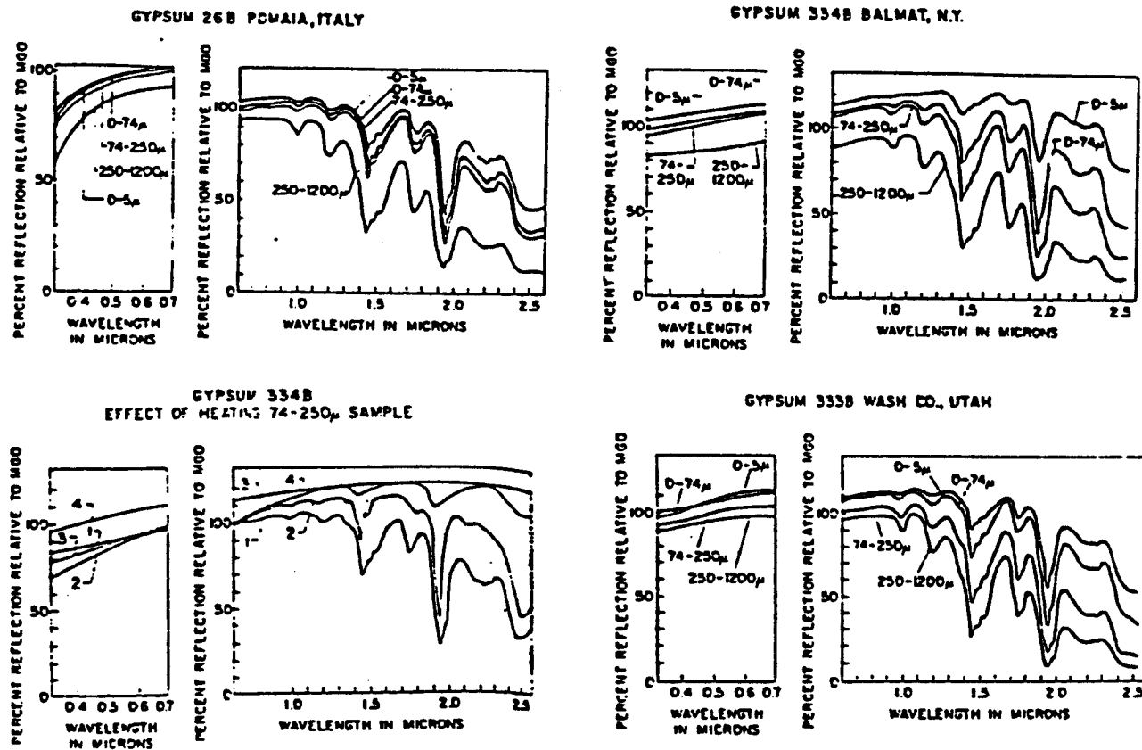
Figure 3. Reflectance characteristics of gypsum from different origins (16).
