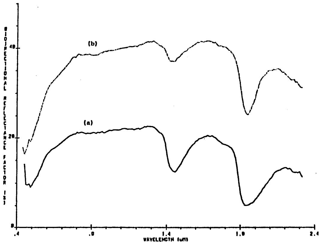
Figure N. The spectral reflectance characteristics for sample Ten (AFTER LEACHING) at (a) saturation and (b) oven dry.
