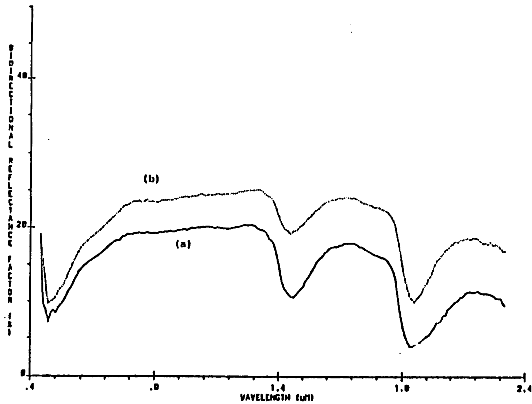
Figure K. The spectral reflectance characteristics for sample Six (AFTER LEACHING) at (a) saturation and (b) oven dry.
