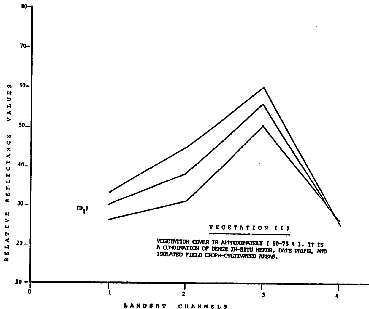
Figure 40. Spectral group B 1 .
