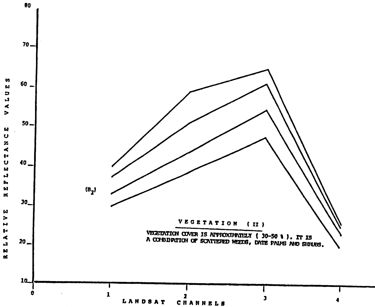
Figure 41. Spectral group B 2 .
