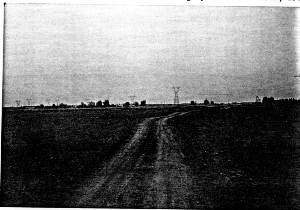
Figure 13. Continuous attraction of moisture from the atmosphere by the soil surface accumulated salts maintains a moist dark brown surface throughout the year. (Photograph: Al-Mahawili, 1981)
