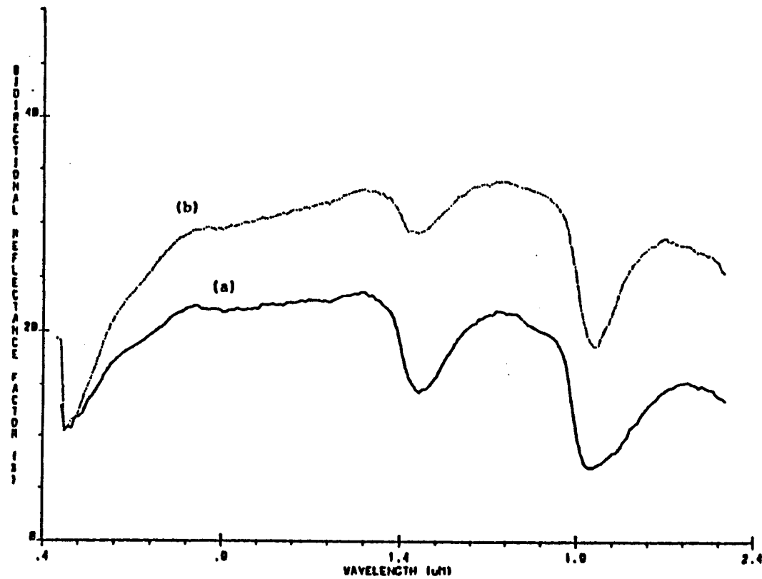
Figure M. The spectral reflectance characteristics for sample Eight (AFTER LEACHING) at (a) saturation and (b) oven dry.
