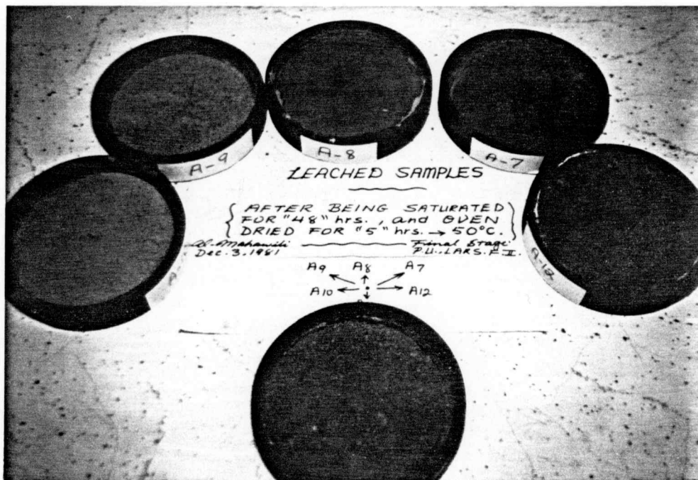
Figure 38. Soil samples 7,8,9,10,11,12 after being leached and oven dried. (Photograph: Al-Mahawili, 1981)
