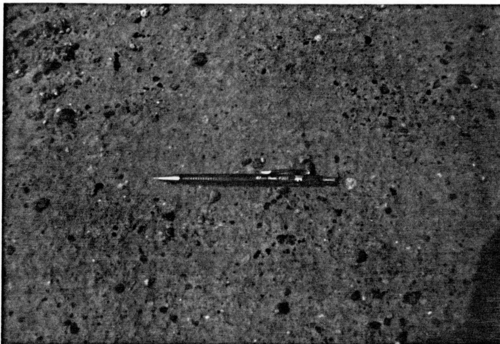
Figure 19. Typical crusted soil surface in gypsiferous soil mixed with gravel and pebbles associated with loamy or sandy textures. (Photograph: Al-Mahawili, 1981)
