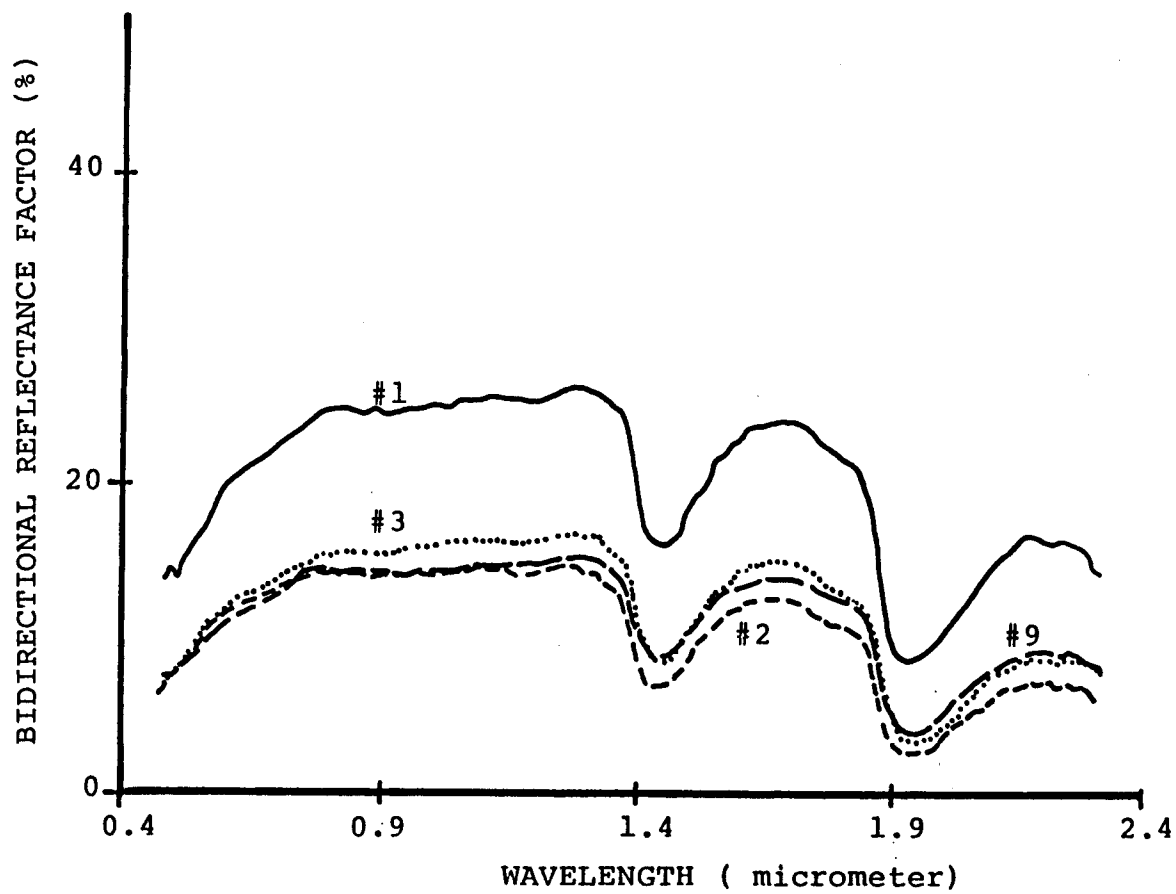
Figure 30. Selected soil samples 1,2,3,9 at the second water content level (2-day air dry) before leaching.
