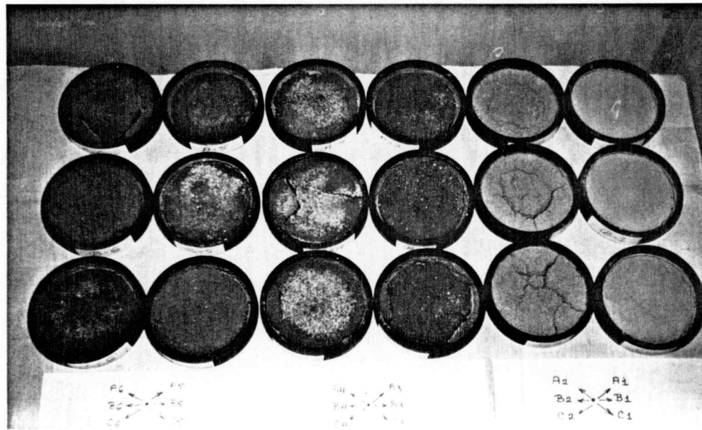
Figure 31. Comparison among different soil surface conditions of soil samples after 6-days of air drying. Notice the non-saline, non-cracked and the homogenization in color of sample 1 (far right) compared with the salt-accumulated, cracked and heterogeneous colors of samples 2,3,4,5,6. (Photograph: Al-Mahawili, 1981)
