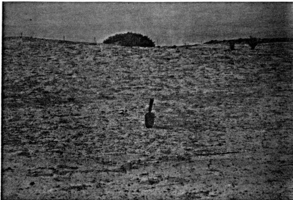
Figure 17. Undulating topography and scattered growth of Prosopis are major land characteristics of the non-saline gypsiferous soils. (Photograph: Al-Mahawili, 1981)
