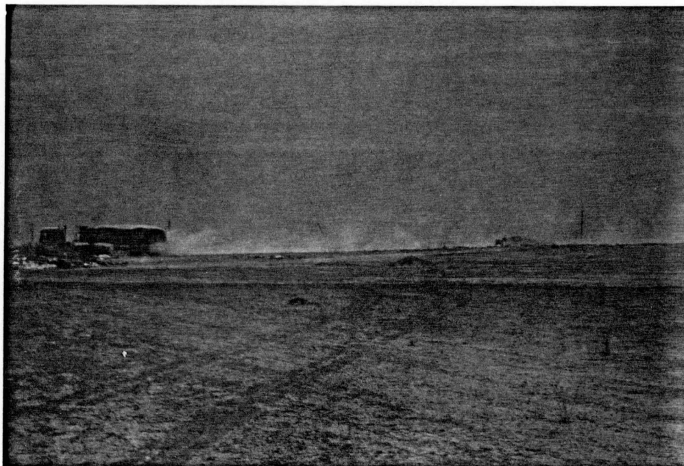
Figure 18. Mining of sand and gravel contributes to severe wind erosion of gypsiferous soils. (Photograph: Al-Mahawili, 1981)
