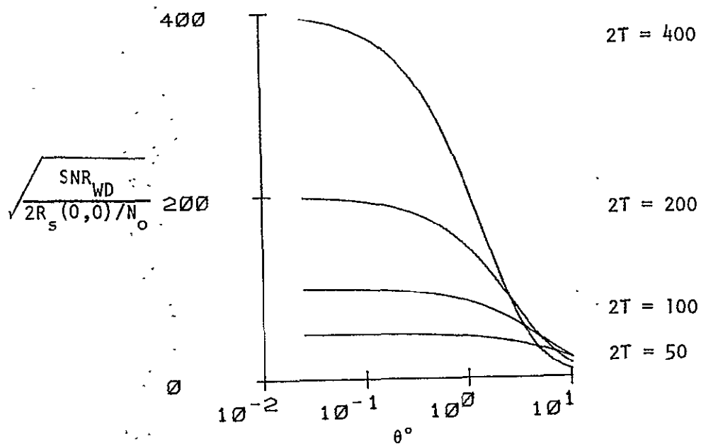
Figure 4-9. (Normalized output signal-to-noise ratio) 1/2 for different integration area sizes vs. rotation angle.
