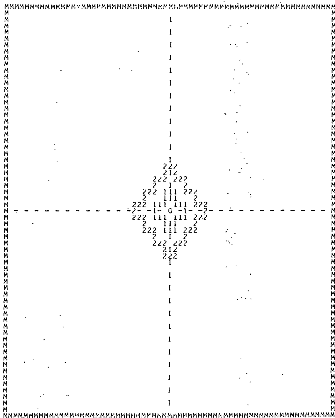
Figure 4-12b. Autocorrelation surface contour for the magnitude of the gradient of the image.
