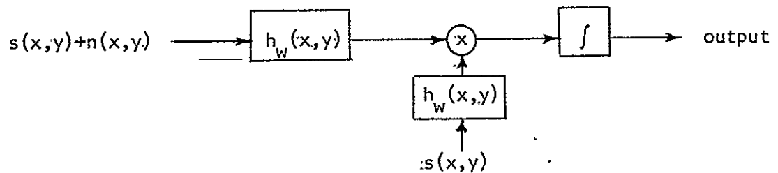
Figure 3-4. Prewhitening representation of matched filter.
