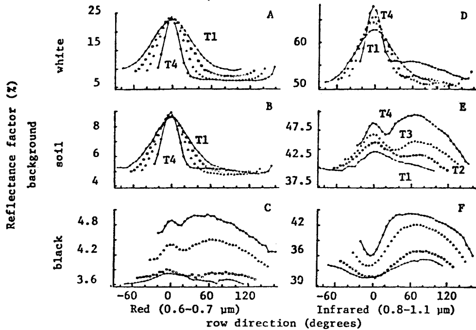
Fig. 3. Soybean canopy reflectance factor with row direction. Zero row direction is the sun azimuth direction. Time periods from solar noon and average sun zenith angles are: T1, -30m to 1h 05, 22°; T2, 1h 05 to 2h 03, 28°; T3, 2h 03 to 2h 23, 34°; T4, 2h 23 to 2h 35, 39°. Canopy had a background cover of 60 percent.
