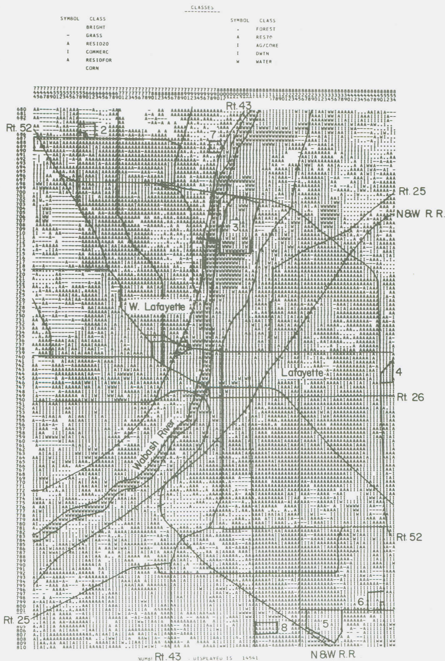
Figure 11. Supervised classification of urban site using spectral data. Same four bands used as in Figure 10. Class symbols explained above printout. Construction sites annotated by numbers 1 through 8.
