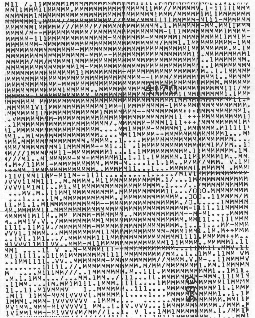
Figure 4 and Figure 5. Enlarged Photo-map Pair, Hayward Area, California. Photo is part of one high altitude color infrared scene acquired at 1:50,000, 15 May 1970, by NASA for USGS Census Cities ERTS experiment. Map is by Purdue/LARS and is based on ERTS-1 scanner digital data for frame 1003-18175, 26 July 1972. Scan lines have been reformatted so that they are nearly parallel to east-west UTM one-kilometer grid lines (zone 10). One printout symbol represents one ERTS scanner picture element (pixel), 0.465 hectare, or 1.1 acres. Urban classes: Commercial-Industrial (I); Mobile Homes (V); Residential (M); Parking Lots (.). Note correspondence between photo and map in mobile home area, lower left corner. Expansion of mobile home park (symbol V on ERTS computer map) is confirmed by NASA 1972 air photo.
