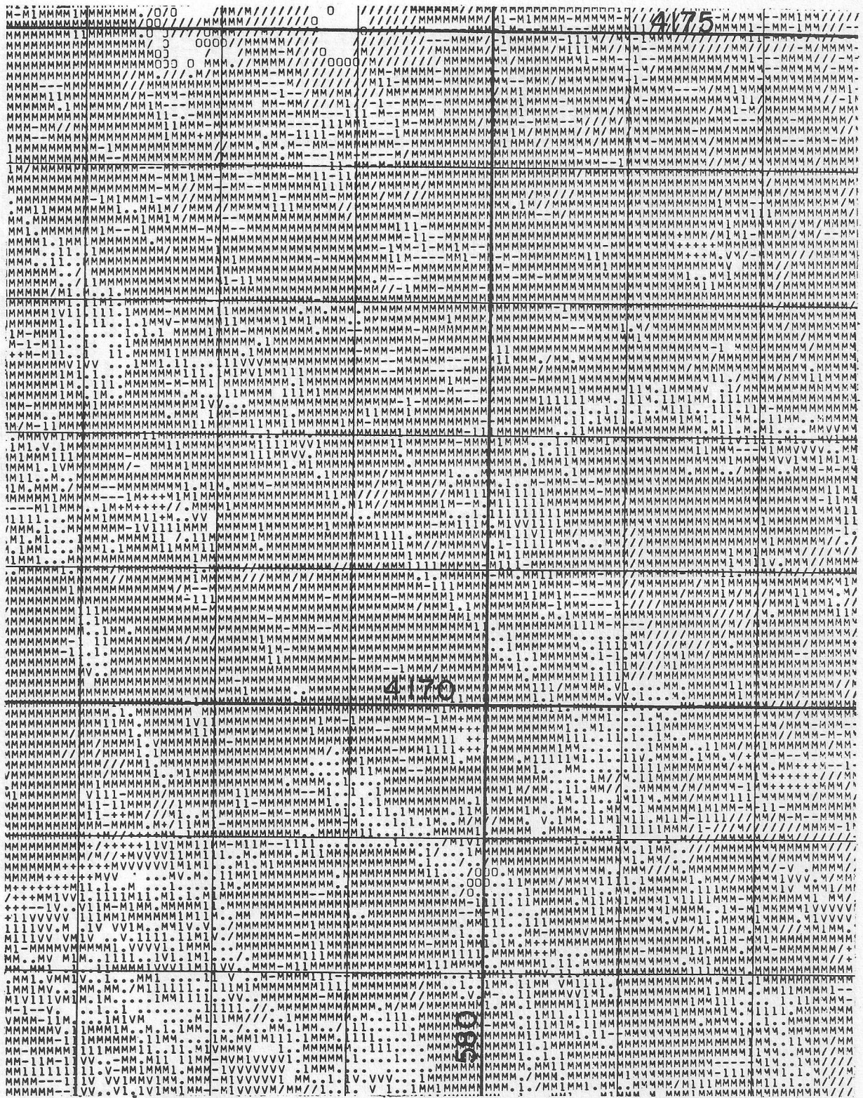
Figure 3. Computer-classified Land-use of the Hayward Area, California. Map is from ERTS-1 scanner digital data for frame 1003-18175, 26 July 1972. Urban classes: Commercial-Industrial (1); Mobile Homes (V); Residential (M); Parking Lots (.); Unimproved open Space, Bare (-); Unimproved Open Space, Trees (/); Open Space-Irrigated (+); Water (0). Approximate orientation of one-kilometer UTM grid (zone 10) indicates scale and direction, and facilitates comparison with corresponding air photo and other ground truth.
