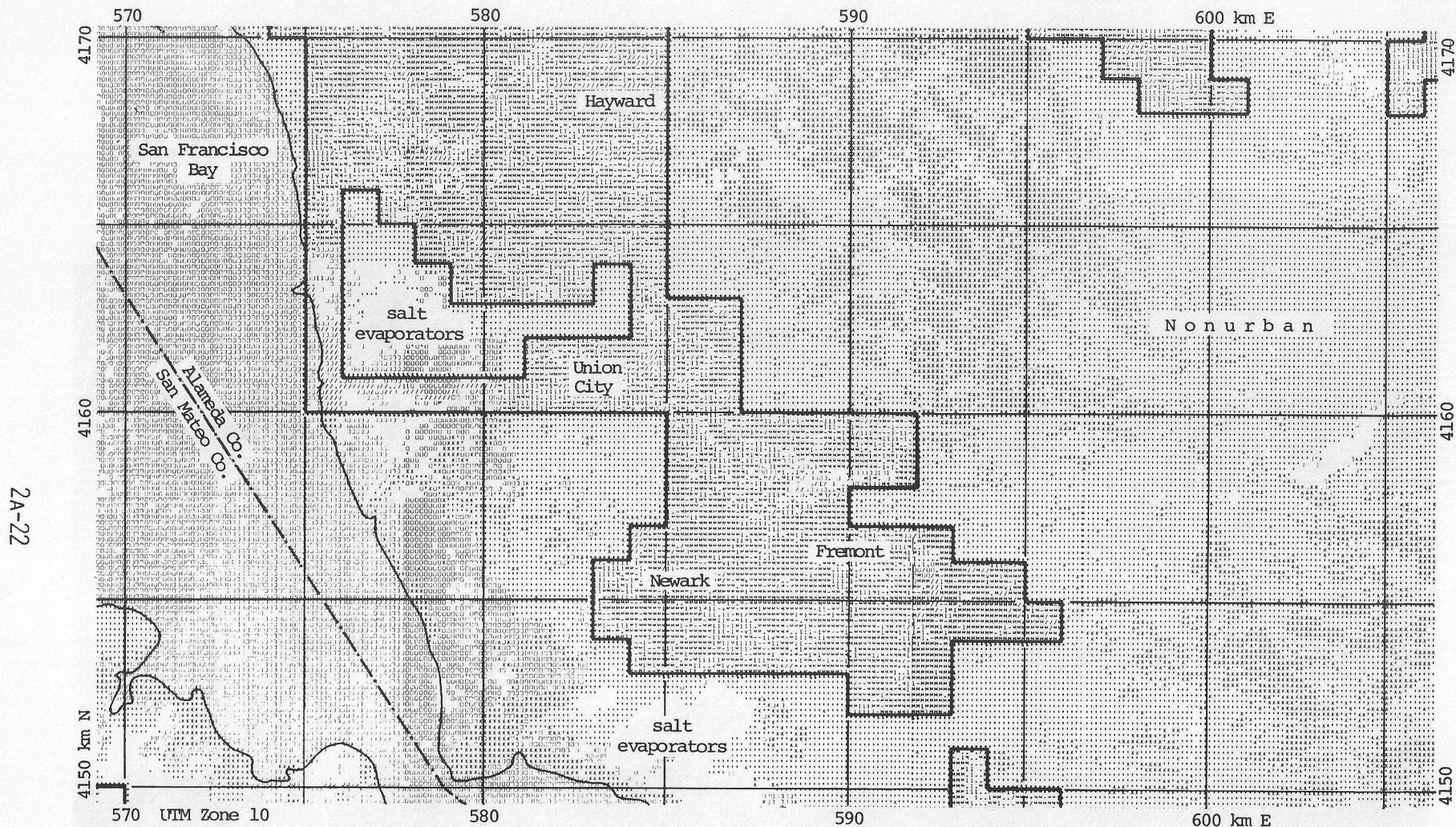
Figure 6b. Portion of computer-classified land use map of San Francisco Bay Region. Map is derived from ERTS-1 scanner digital data, frame 1003-18175, 26 July 1972. Classification, by Purdue/LARS, uses eight Urban classes, and three Nonurban classes (Figures 4 and 5). Urban area, defined by one-kilometer UTM grid (Zone 10), is from USGS Census Cities ERTS experiment and NASA aircraft photography. The grid facilitates comparison with corresponding ERTS-1 RBV scene (Figure 6a). Map is produced at 1:48,000 by classifying every other pixel in every other scan line. About 6500 square kilometers (or just under one-tenth of one percent of U.S. land area) were classified on LARS IBM 360-67 in about thirty minutes' computer time. Aggregation of areas by land use class and kilometer grid square can also be generated. It may soon be operationally and economically feasible to compile manuscript land use maps for large areas by this method, using additional Nonurban classes. Then edit and adapt to more conventional functional classes. Perhaps, draw use boundaries by conventional cartography or computer graphic methods, and publish maps at 1:50,000 to 1:250,000. Area measurement and land use change data by grid cell, or user jurisdiction area, would be valuable by-products. (-Ellefsen, Swain, and Wray, Figure 6b)
