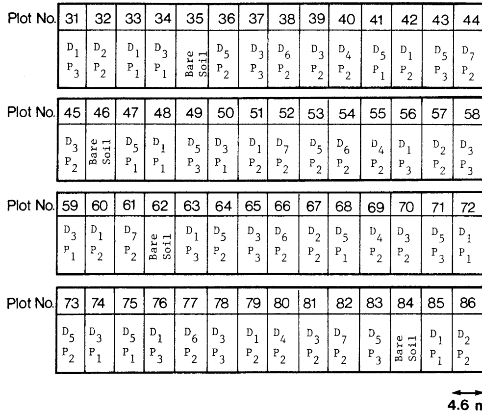
Figure B-2. Design and treatment descriptions of the 1980 Purdue Agronomy Farm Corn Cultural Practices Experiment.
