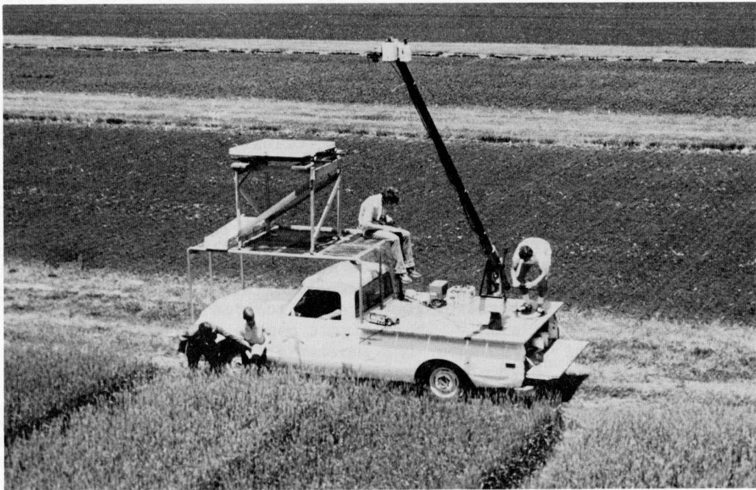
Figure A-3.1 Field radiometer system including Exotech Model 100 radiometer, camera, and \text{BaSO}_4 calibration standard.
