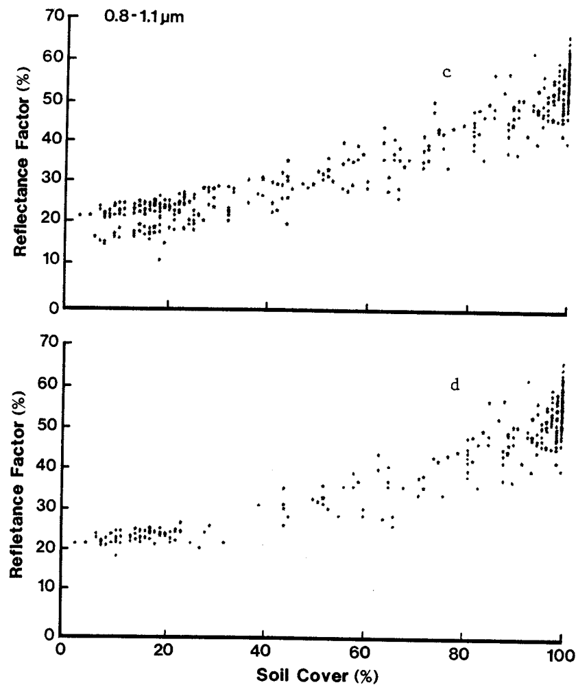
Figure A-5.1. Time of day effect on the RF seen in the 1978 data for the red (0.6-0.7 \mu\text{m} ) and the near infrared (0.8-1.1 \mu\text{m} ) wavelength regions. (a,c) All 1978 data minus dates which include wet soil and/or senescing vegetation. (b,d) Same as a and c above, but only includes data in the three hour time period centered about solar noon.
