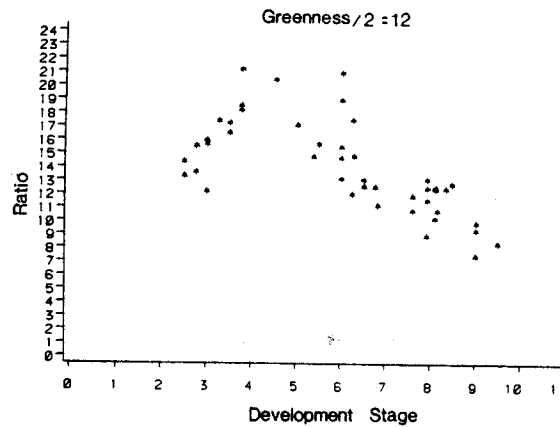
Figure A-2.14. Example relationships of red and near infrared ratio values and development stage for corn greenness response levels of 2, 8, and 12 showing potential increase in information over using greenness alone.
