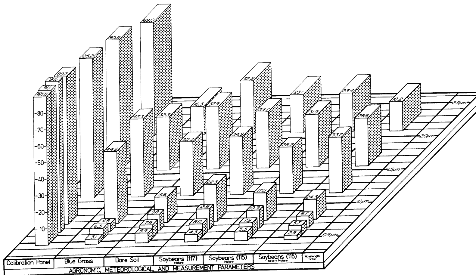
Figure C-11. Reflectance factor data acquired by the multiband radiometer for several cover types.
