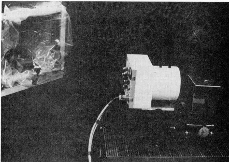
Figure C-6. Chamber and source used for environmental performance tests of the thermal channel.
