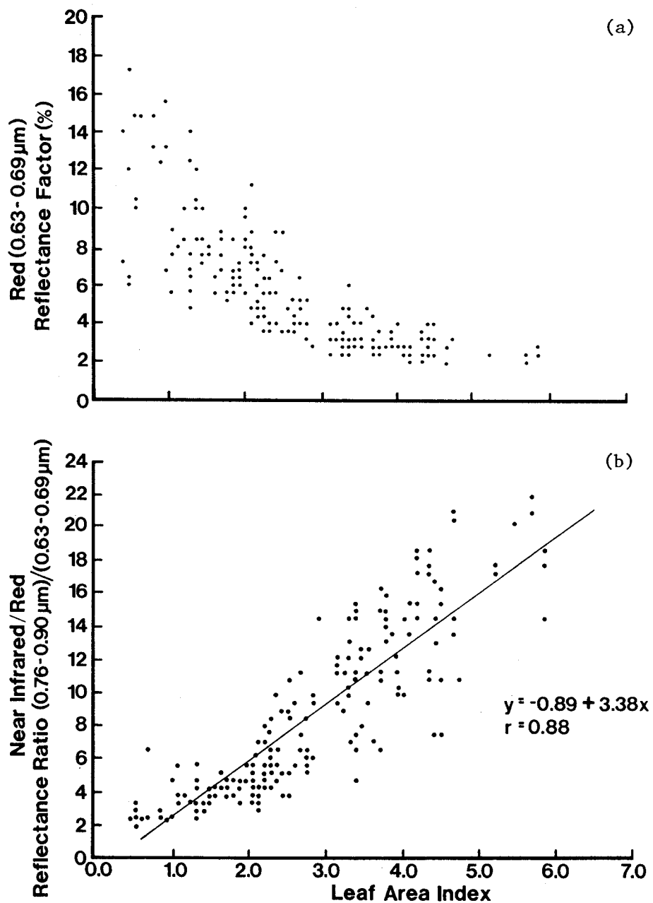
Figure A-4.4. The relationship of (a) the red (0.63-0.69 \mu\text{m} ) reflectance factor and (b) the near infrared/red reflectance ratio, (0.76-0.90 \mu\text{m} )/(0.63-0.69 \mu\text{m} ), to leaf area index. Both 1978 and 1979 data are included.
