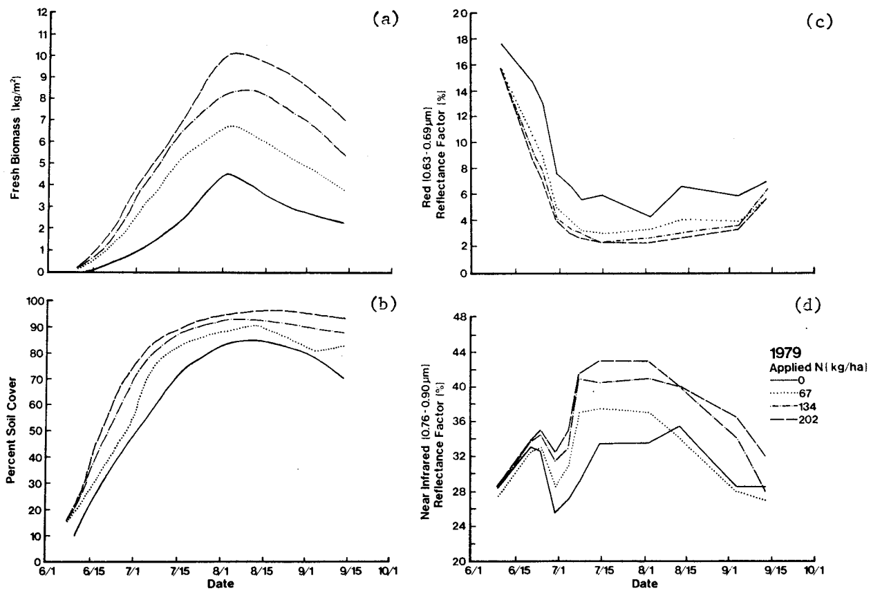
Figure A-4.3. Temporal changes in (a) fresh biomass, (b) percent soil cover, (c) red (0.63-0.69 \mu\text{m} ) and (d) near infrared (0.76-0.90 \mu\text{m} ) reflectance factor for maize canopies under four N treatment levels in 1979.
