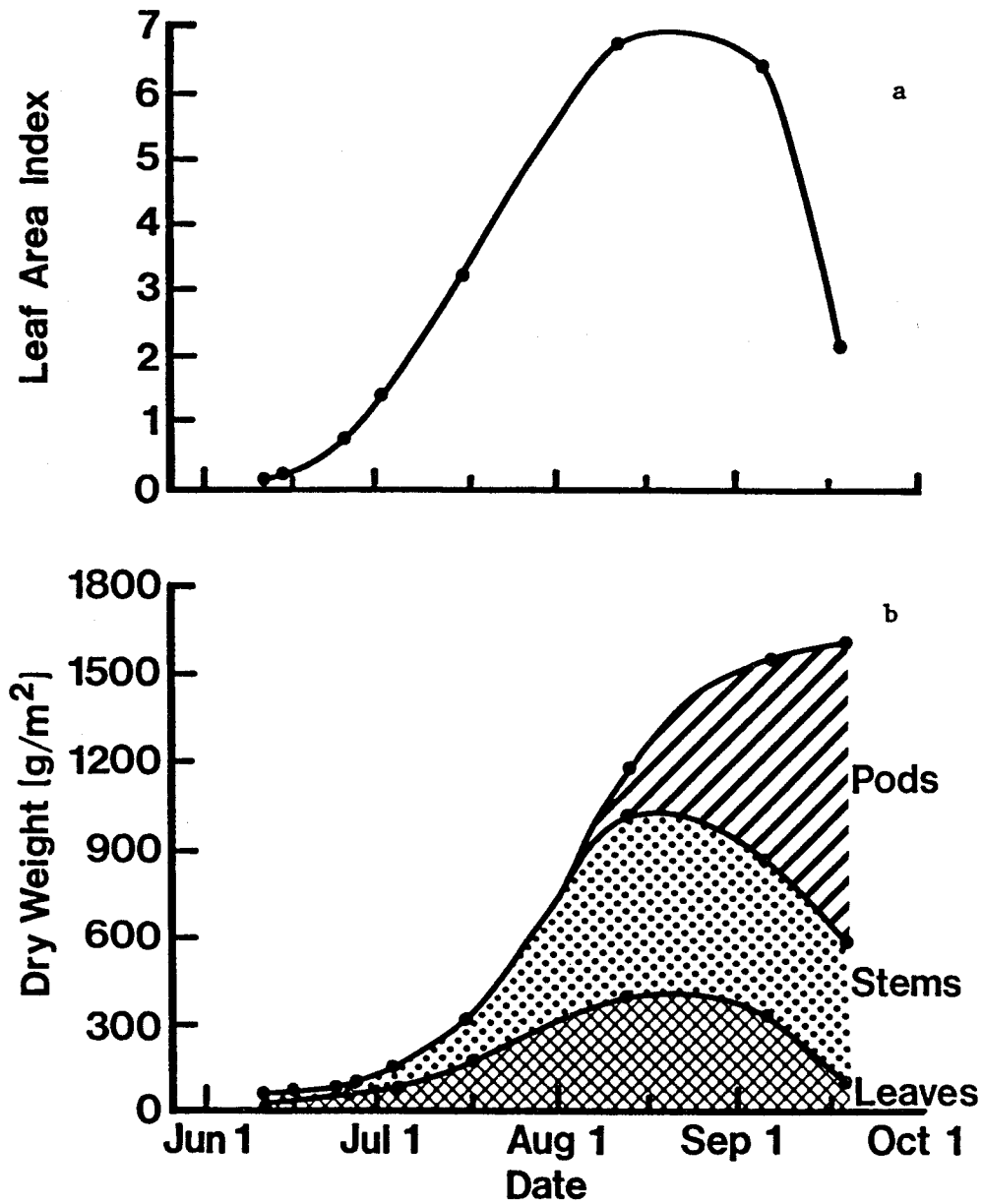
Figure A-3.4. Seasonal changes in (a) leaf area index and (b) soybean canopy components for the May 24 planting date on Chalmers silty clay loam.
