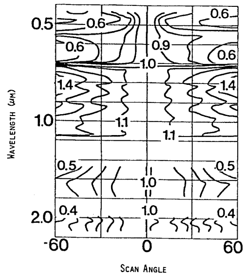
Figure A-6.4. Simulated, normalized reflectance factor for a multispectral line scanner plotted in topographic notation with contour lines at 0.1 intervals. In this example from noon on 17 July 1976 the aircraft is flying toward the sun. This same coordinate system is used in each of the 24 plots in Figures A-6.5 and A-6.6.
