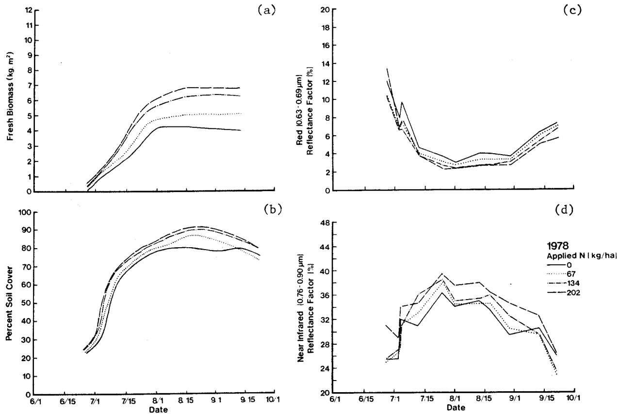
Figure A-4.2. Temporal changes in (a) fresh biomass, (b) percent soil cover, (c) red (0.63-0.69 μm) and (d) near infrared (0.76-0.90 μm) reflectance factor for maize canopies under four N treatment levels in 1978.
