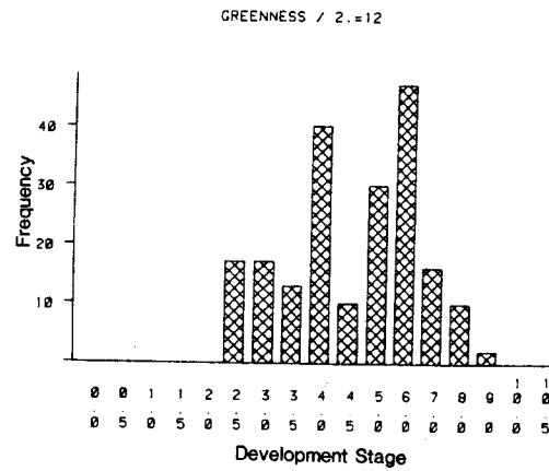
Figure A-2.10. Histograms of development stage for greenness levels of 2, 8, and 12 representing greenest response ranges of 3-5, 15-17, and 23-25 units respectively. These examples for corn illustrate multi-modal and widely dispersed distributions.
