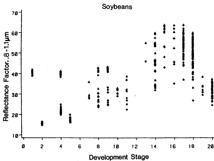
Figure A-2.3. Relationships of near infrared (.8-1.1 \mu\text{m} ) reflectance and development stage of corn and soybeans.
