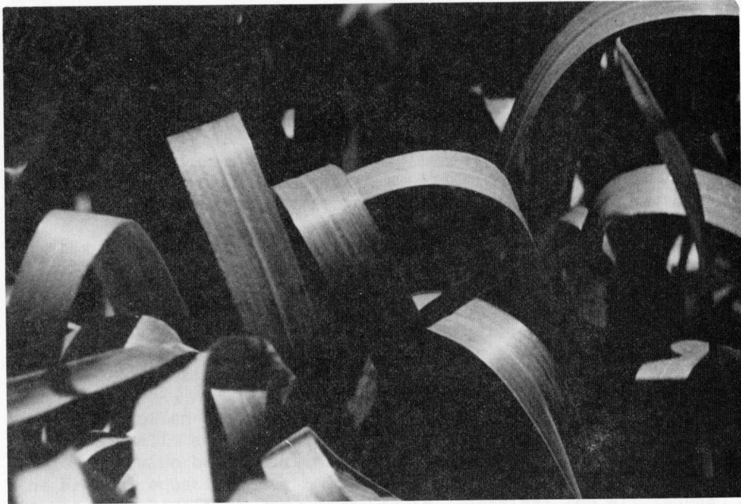
Figure A-7.1. Specular Reflection. The camera received specularly reflected sunlight from the bright areas of these wheat flag leaves.
