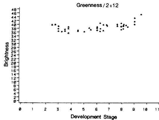
Figure A-2.15. Example relationships of transformed brightness values and development stage for corn greenness response levels of 2, 8, and 12. The increase in information is not as apparent as in Figure A-2.14.
