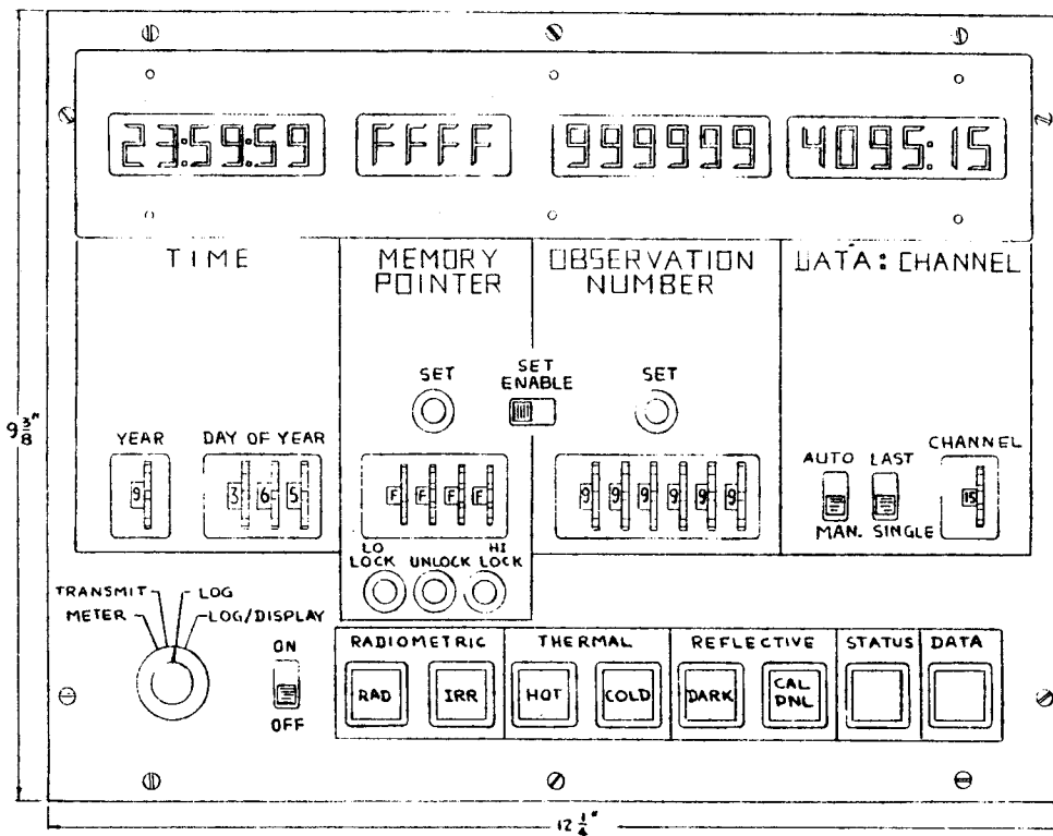
Figure C-14. Front panel controls and displays of prototype data logger.
