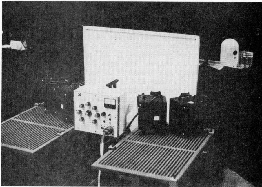
Figure C-5. Laboratory set-up for linearity tests.
