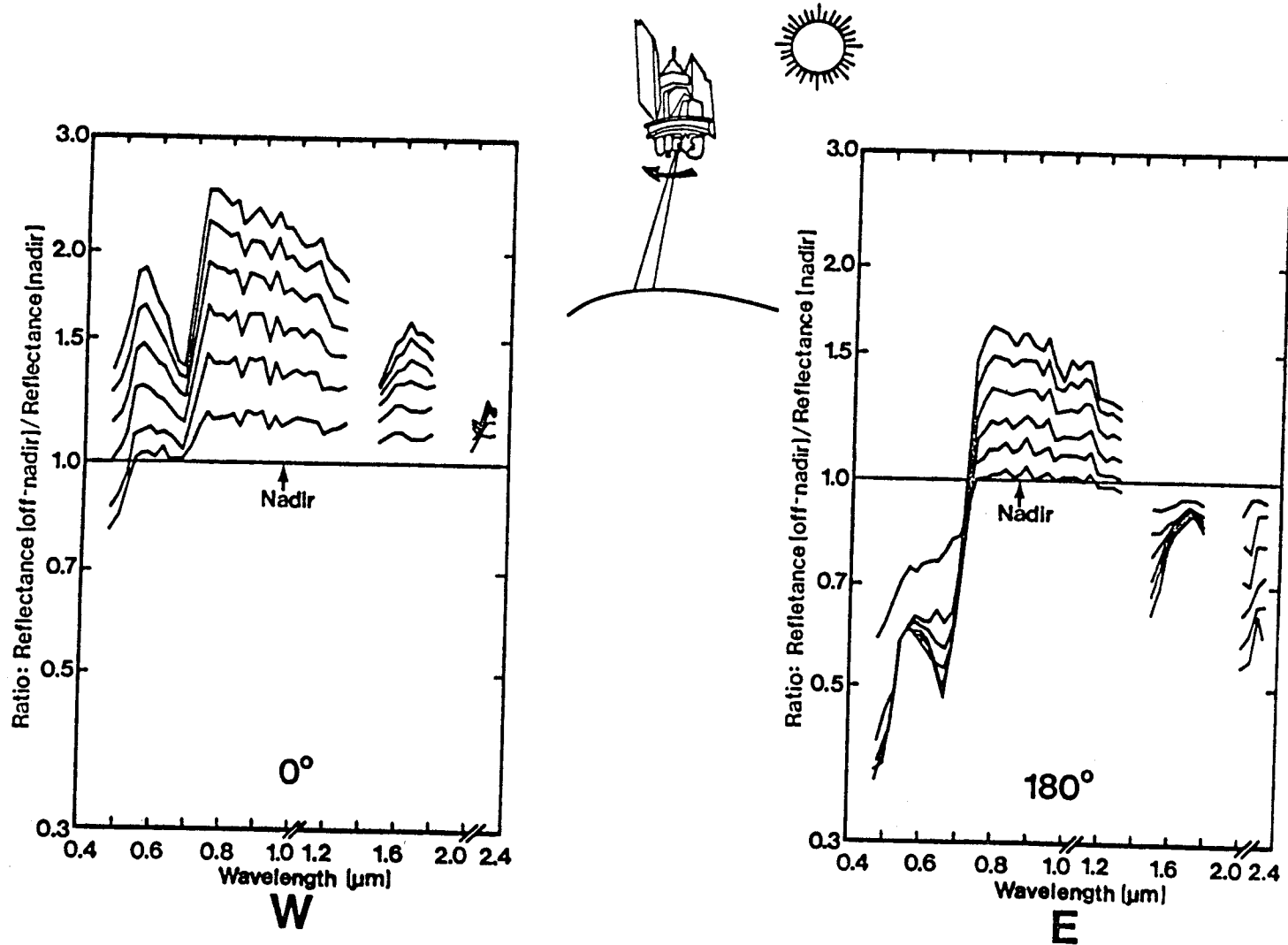
Figure A-6.2. Normalized reflectance factor of spring wheat three hours before solar noon on 21 June 1976 with view azimuths of 0^\circ (west) and 180^\circ (east). Solar azimuth was 43^\circ zenith, 109^\circ azimuth.
