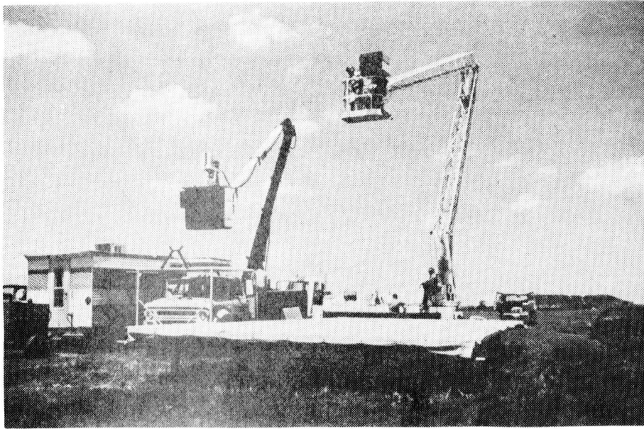
Figure F-11. Purdue/LARS Exotech 20C (left) and NASA/JSC FSAS (right) spectrometer systems viewing canvas panel.
