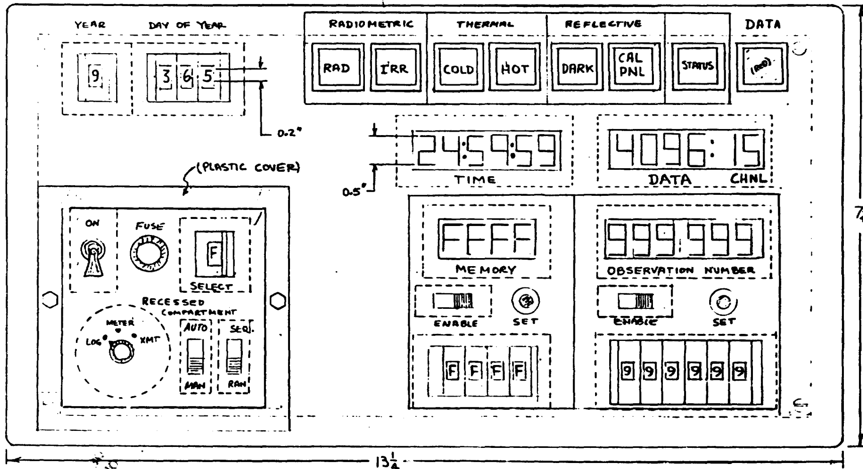
Figure C-5. Sketch of Front Panel of Data Recording Module.
