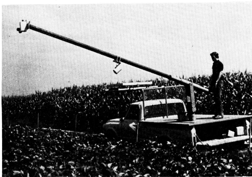
Figure F-1. Truck-mounted multiband radiometer viewing a soybean canopy.
