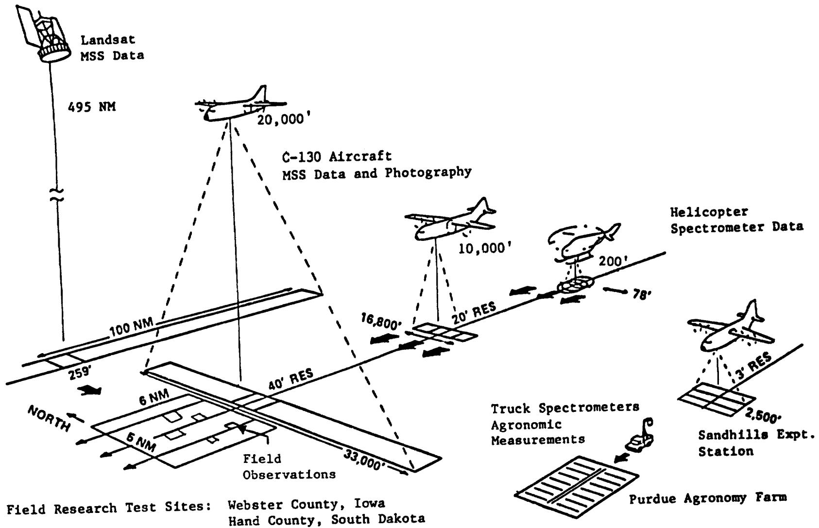
Figure A-2. Schematic illustration of multistage approach to multicrop field research data acquisition.
