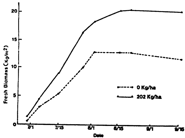
Figure A-9. Effect of nitrogen fertilization on percent soil cover, leaf area index, fresh biomass and plant nitrogen content of corn canopies as a function of measurement date.
