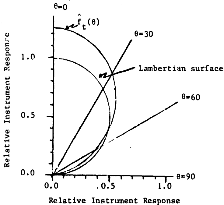
Figure F-9. Polar plot of comparison of relative response of a normal viewing instrument to a scene characterized by \hat{f}_t and a Lambertian scene as a function of illumination angle, \theta .
