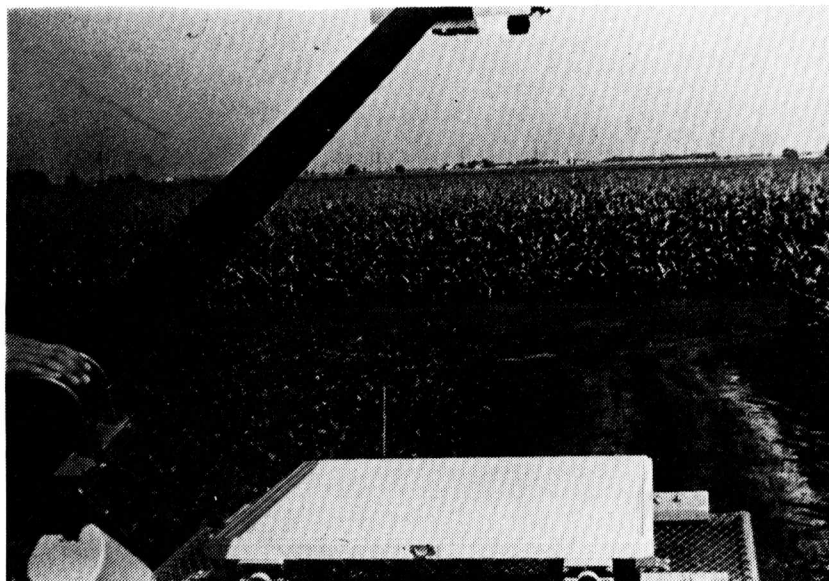
Figure F-2. Multiband radiometer positioned over painted barium sulfate reference panel for field reflectance calibration.
