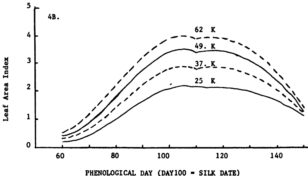
Figure B-4. The solar radiation intercepted ( SR_{Int} ) by a corn canopy was estimated as a function of leaf area index and total solar radiation (SR) received on a horizontal surface. The average seasonal leaf area index curves (B-4B) were visually smoothed from experimental data for 25,000, 37,000, 49,000, and 62,000 corn plants per hectare (from Dale and Hodges, 1975).
