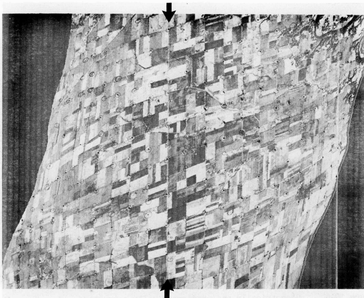
Figure 16-5. Same data as in Figure 16-4 after a north-south road was straightened to compensate for aircraft roll and after scan lines were resampled to compensate for aircraft pitch.
