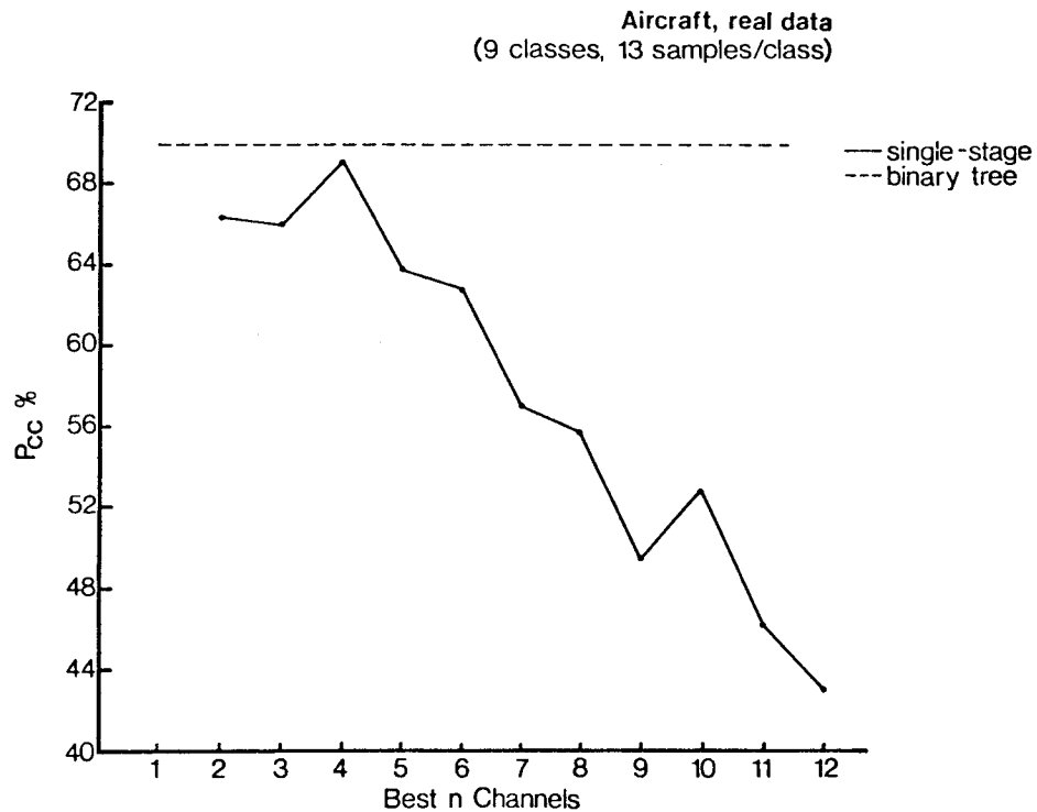
Figure 10-4. Single-stage and binary tree classification results for the aircraft data set.
