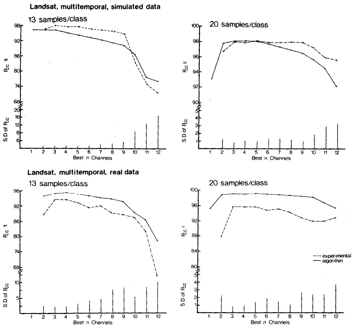
Figure 10-3. Experimental and algorithm results for simulated and real multitemporal Landsat data with two sizes of training sets.
