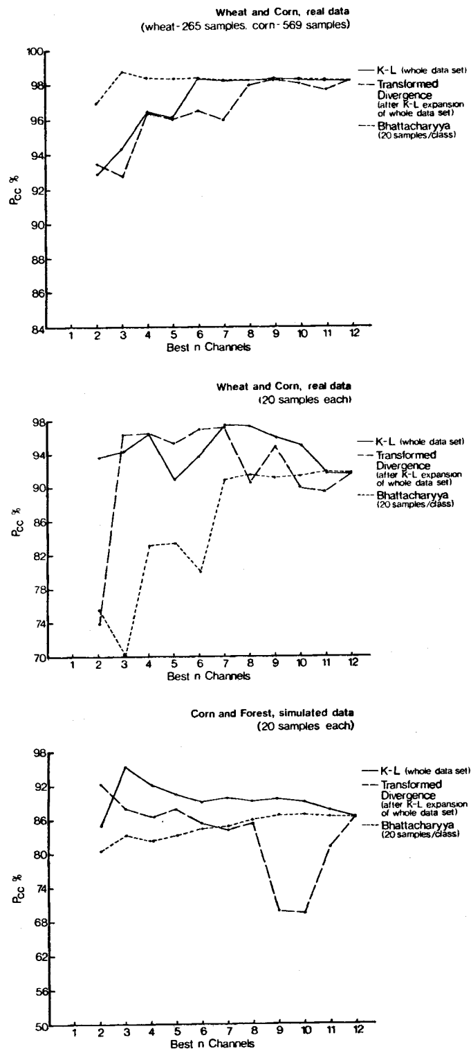
Figure 10-1. Experiments on feature selection using a large number (top) and a small number (middle and lower) of training samples.
