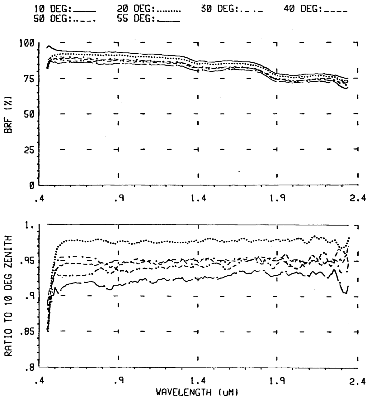
Figure 3-1. Example graph of bidirectional reflectance factor (BRF) calibration of barium sulfate reflectance reference panel that is sent with panel to field research test sites.
