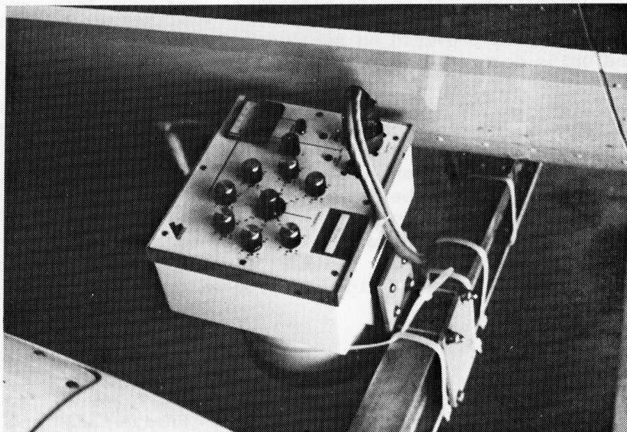
Figure 4-2. Model 12-1000 multiband radiometer mounted on helicopter for test.
