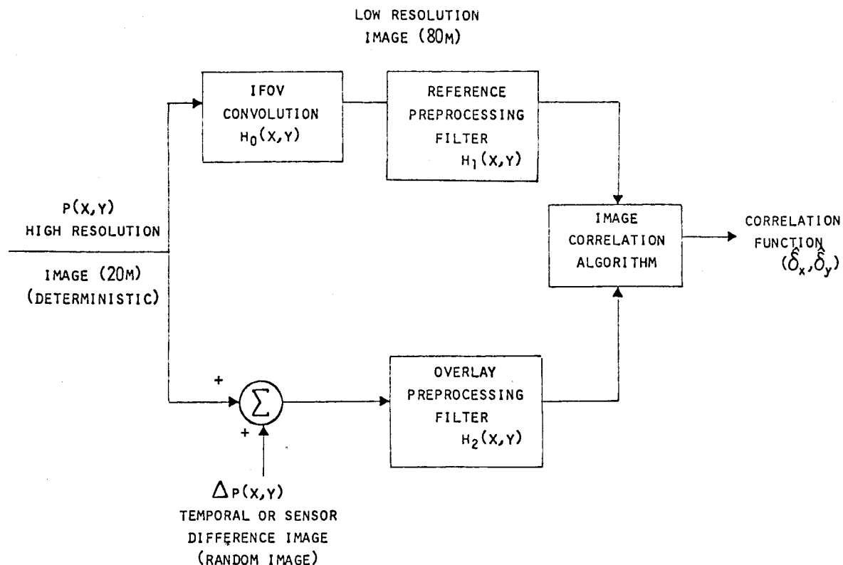
Figure 13-1. Model for analysis of registration of data with different spatial resolutions.
