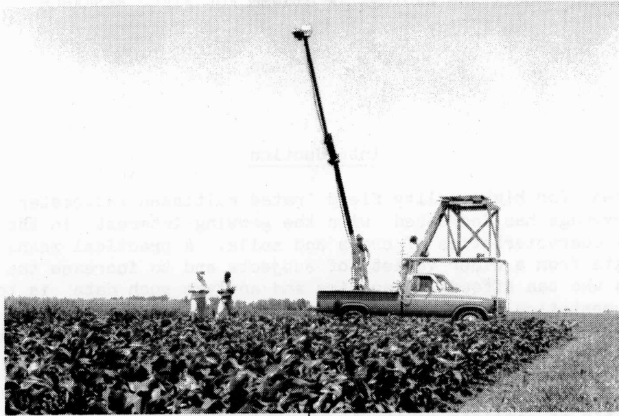
Figure 4-1. Pickup truck data acquisition system, with boom, multiband radiometer, camera, data logger, calibration tower and panel.
