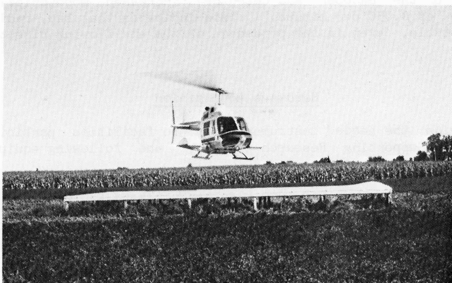
Figure 4-3. Helicopter with Model 12-1000 radiometer over calibration panel.
