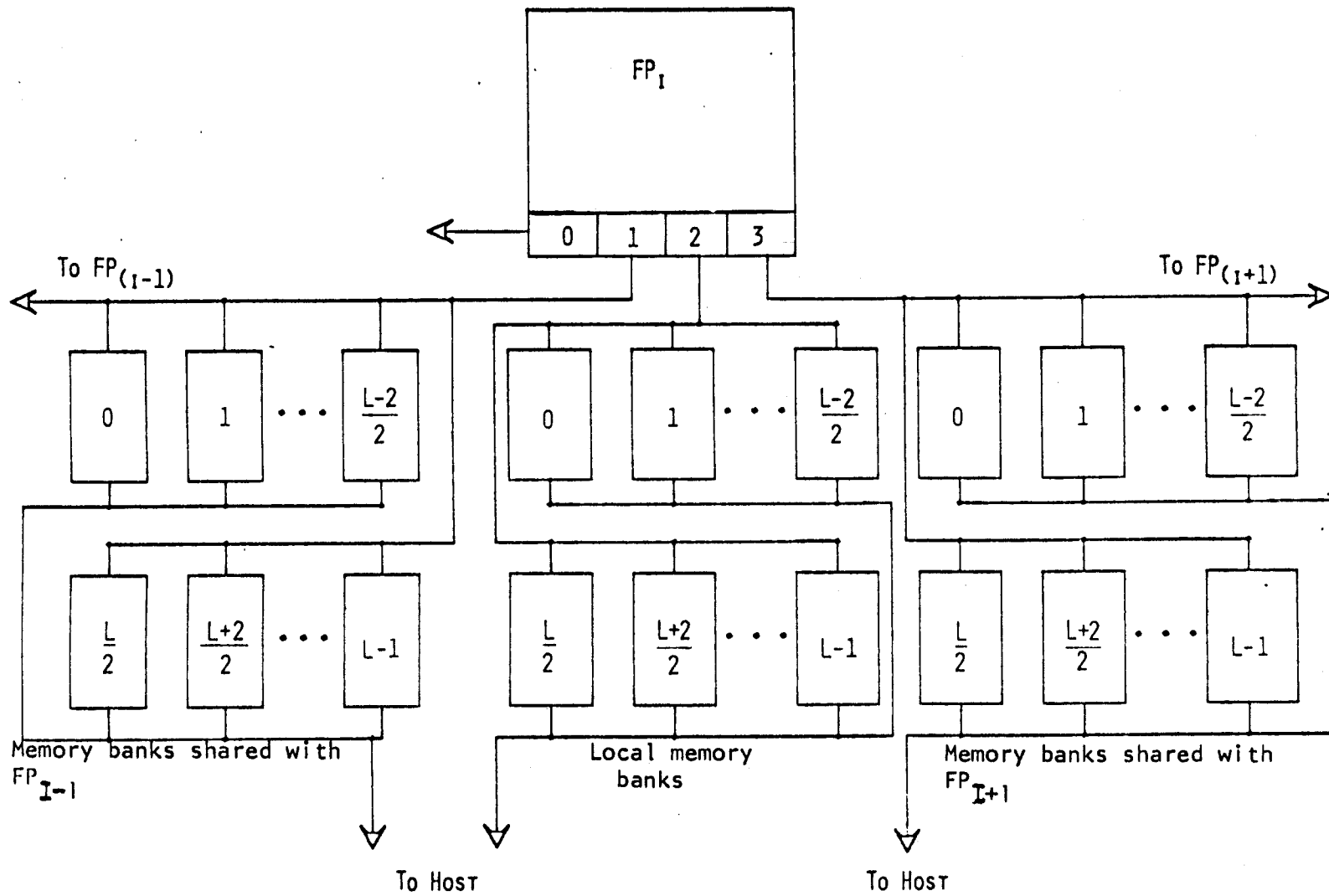
Figure 11-5. Potential memory organization for striping scheme.
