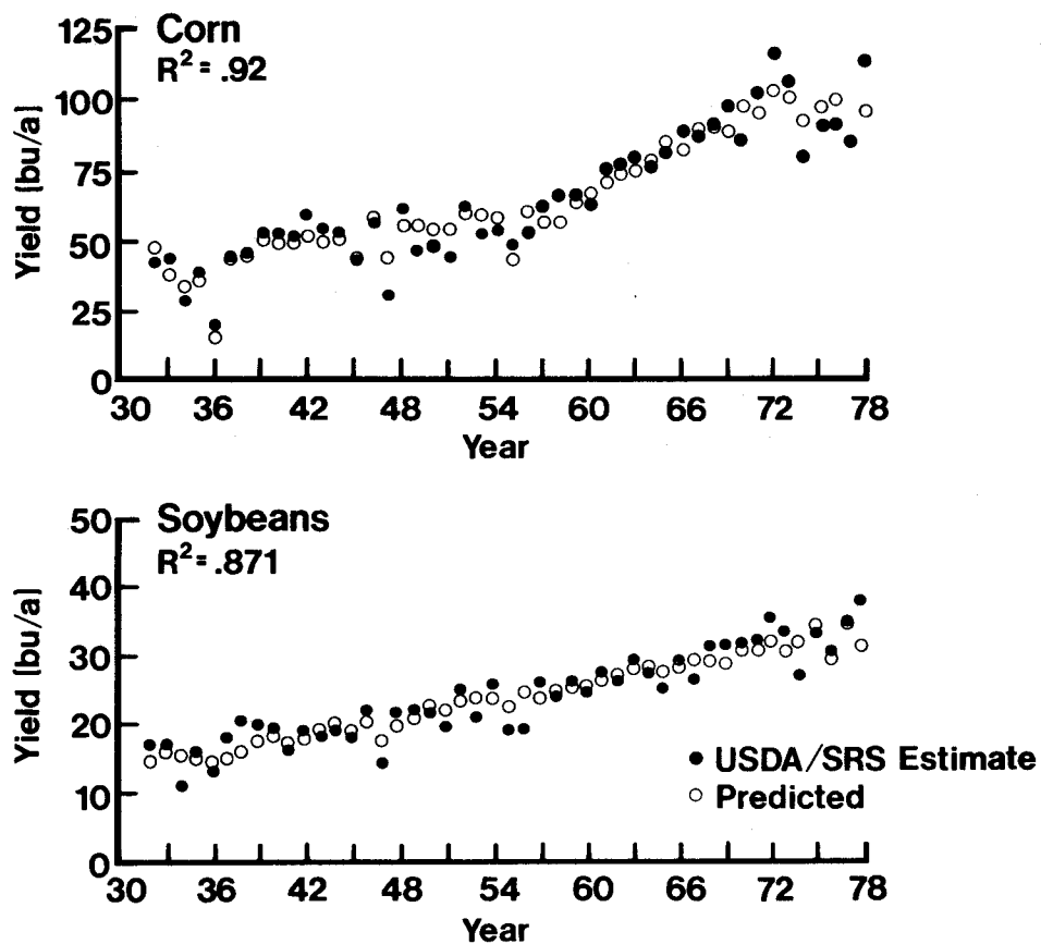
Figure 9-2. Comparison of corn and soybean yields predicted by the regression equations of historical weather data and the USDA/SRS estimates for the entire state of Iowa.
