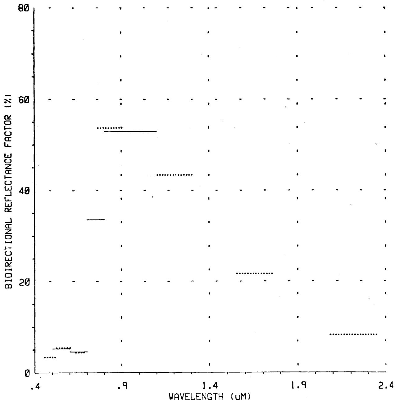
Figure 3-2. Graph of Exotech 100 Landsat band and Barnes 12-1000 Thematic Mapper band radiometer data illustrating plotting of reflectance data with different wavelength resolutions on the same graph.
