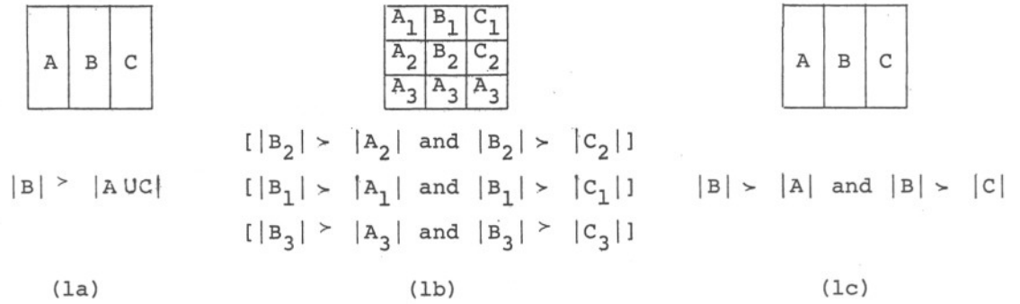
Figure 1. Description of the linear (1a), the nonlinear (1b), and the semilinear (1c) detectors for the vertical case.
