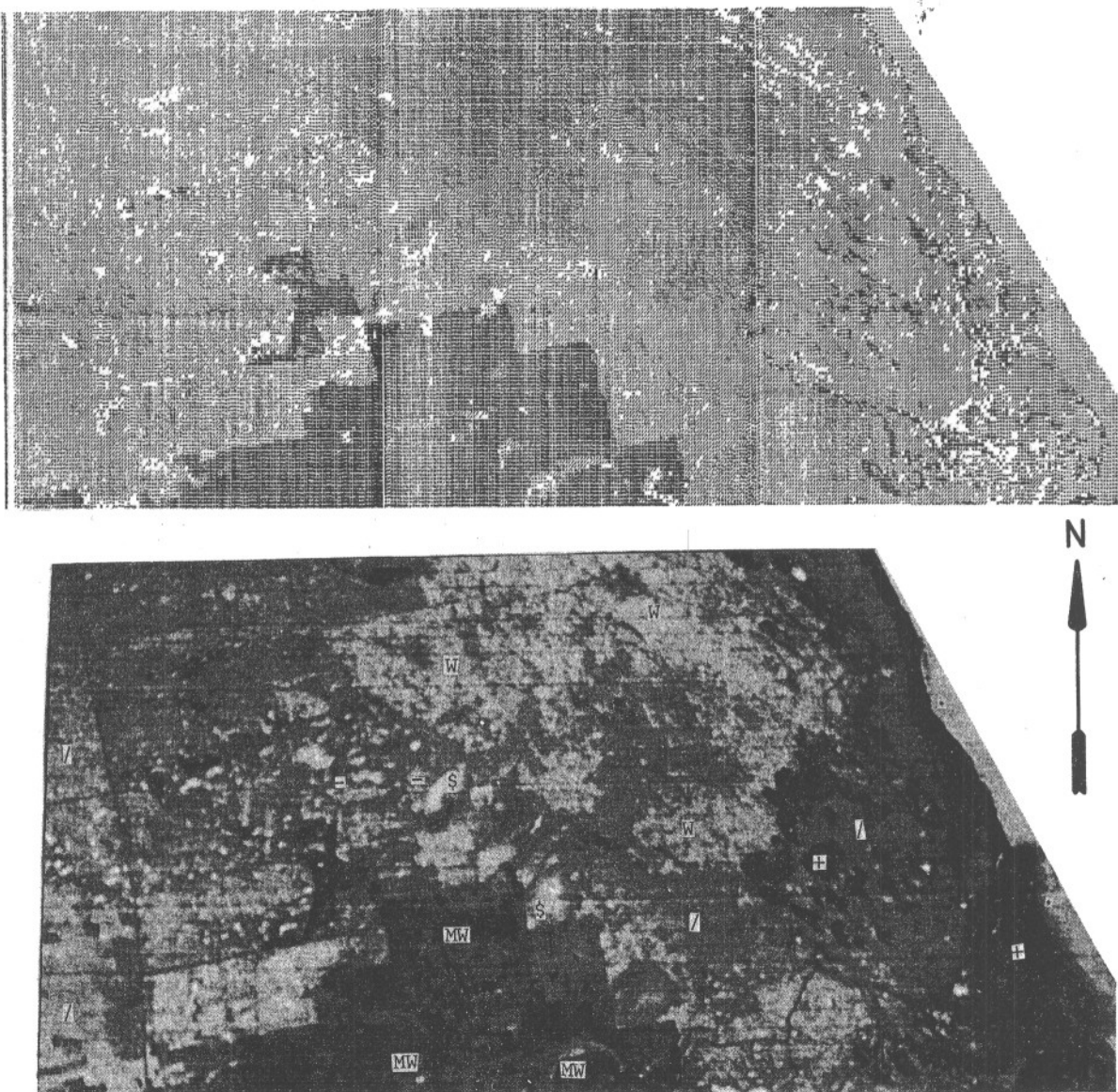
Figure 1. Black-and-white print using MSS 5 (lower) and line printer classification map (upper) of the 81,000-ha rangeland area in Kenedy and Willacy Counties of south Texas for the October 17, 1975 LANDSAT-2 overpass. Resolution of classification map is 1.9 ha/symbol. Definition of land-use category symbols are: live oak rangeland (W), mixed brush rangeland (/), grasslands (-), barren land (+), wetland ($), agricultural land (M overprinted with a W), water (•), and threshold (blank).
