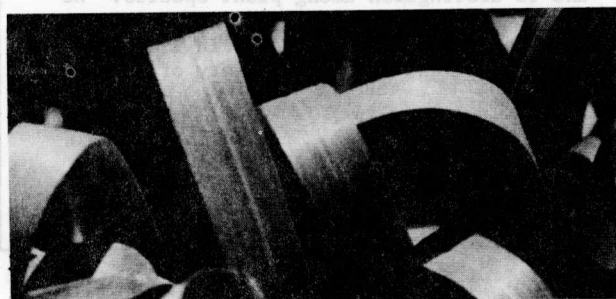
Figure 1. Specular Reflection. The camera received specularly reflected sunlight from the bright areas of these wheat flag leaves.
