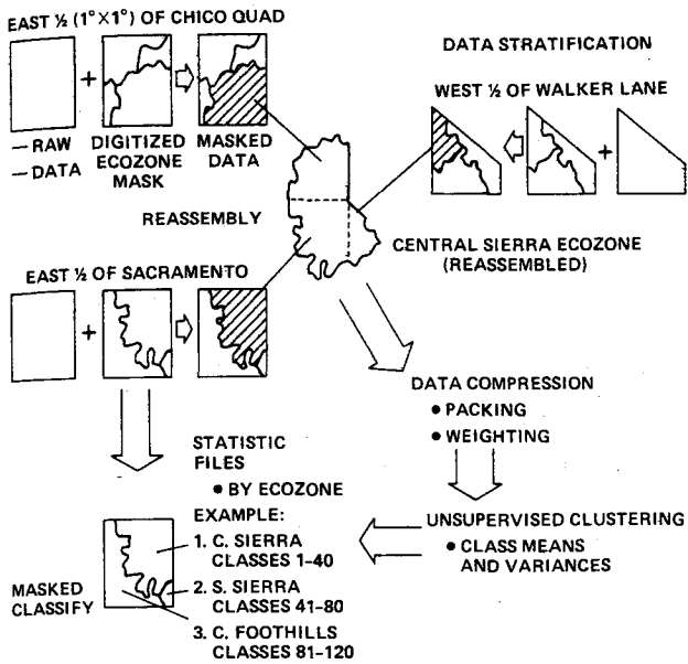
Figure 6. Classification Processing.
