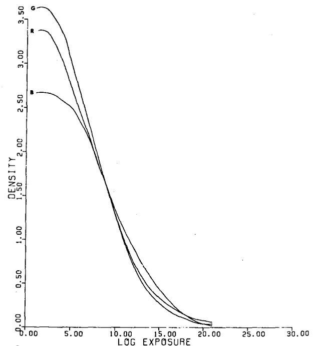
Figure 1. D-LOG E CURVES
