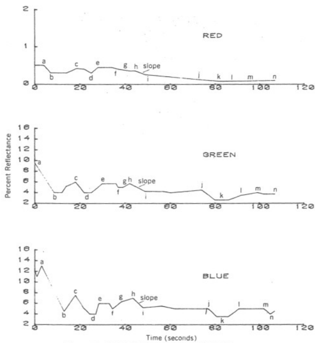
Figure 6. ANALOG REFLECTANCE DATA
