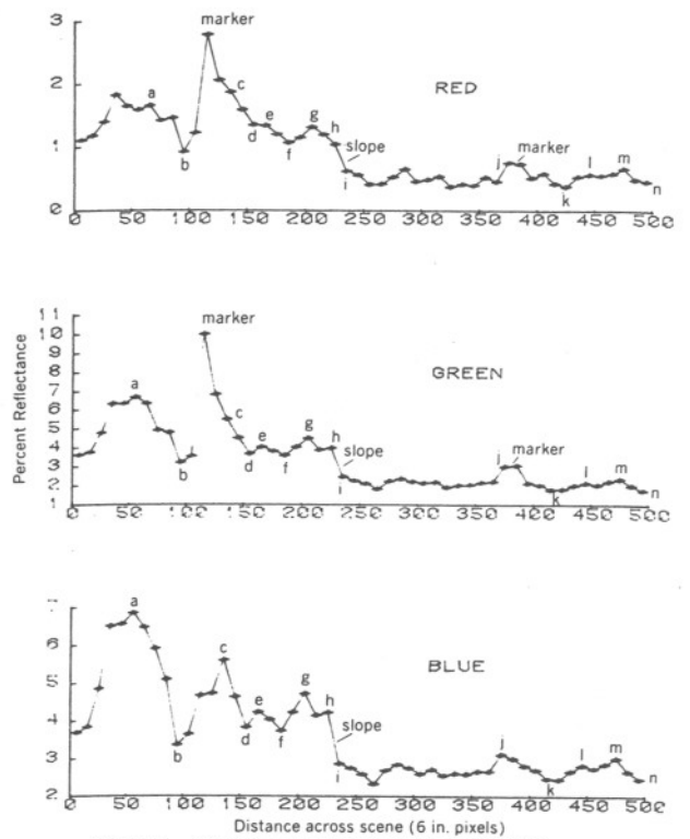
Figure 8. AVERAGE DERIVED REFLECTANCES
