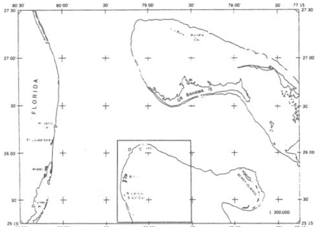
Figure 2 BAHAMAS PHOTOBATHYMETRIC CALIBRATION RANGE
